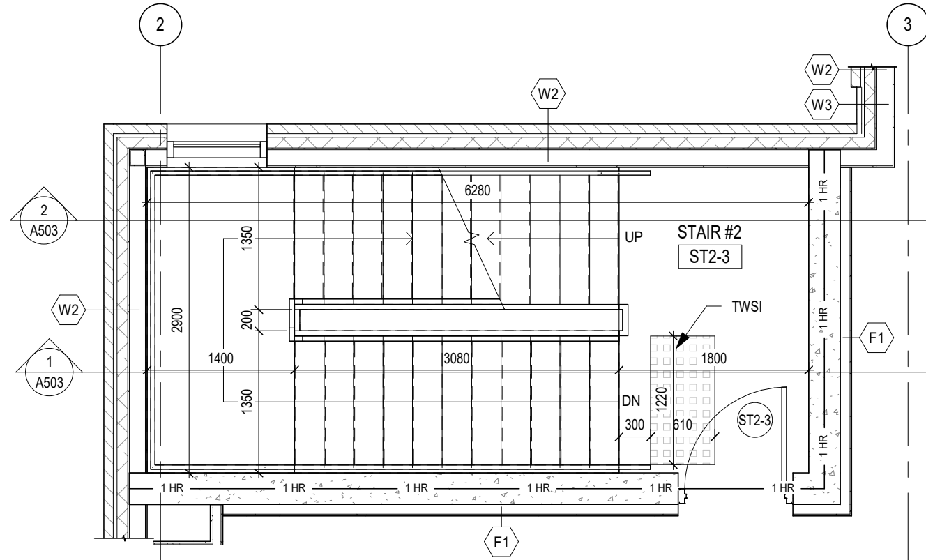
8 STAIR #2 - 3rd FLOOR PLAN A501 1 : 50
