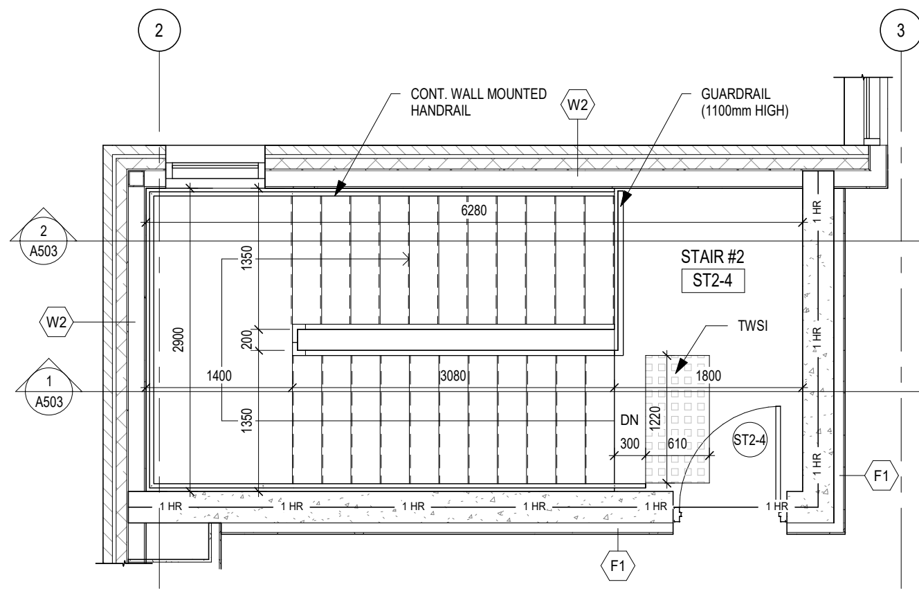
9 STAIR #2 - 4th FLOOR PLAN A501 1 : 50
