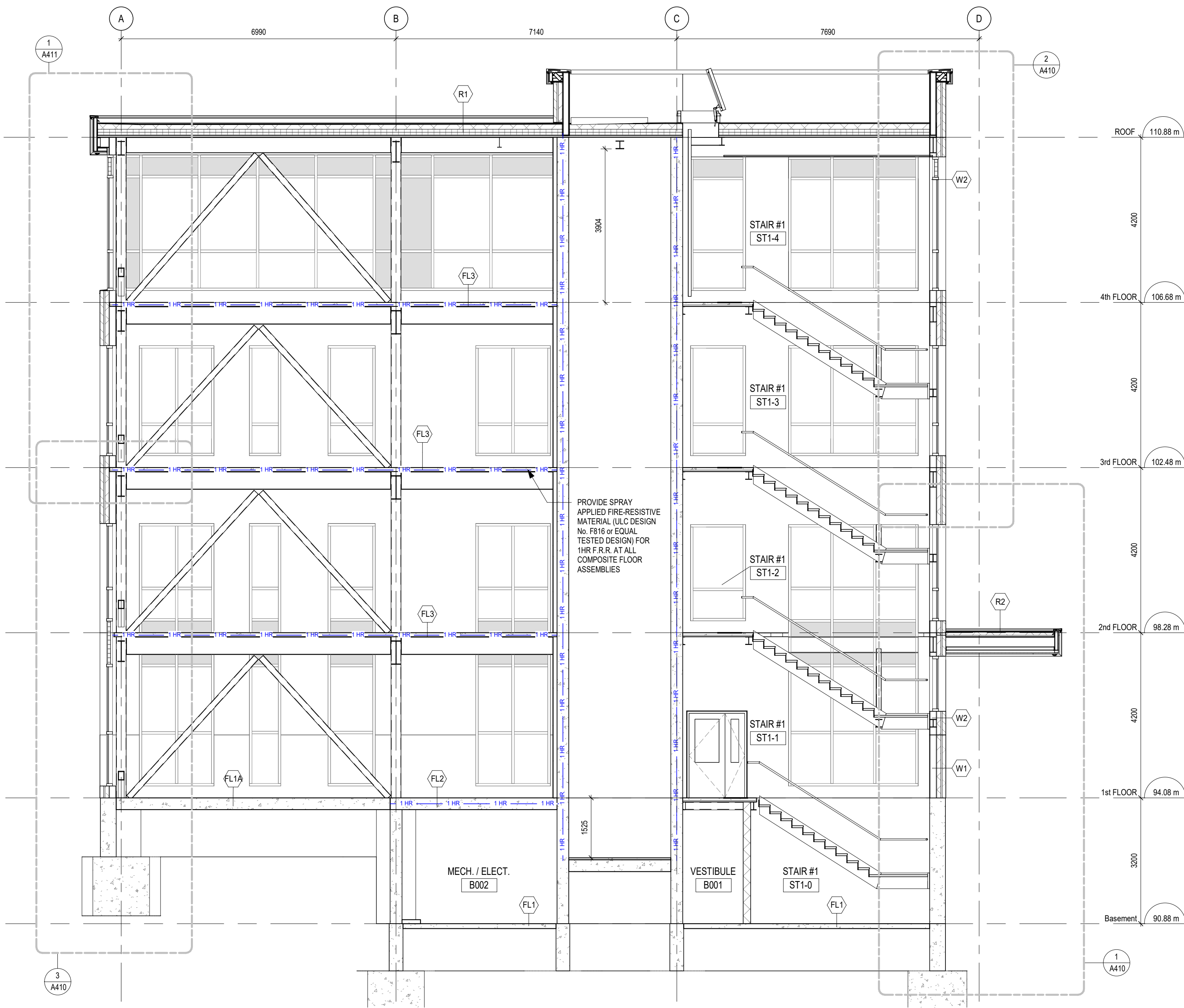
1 BUILDING SECTION A401 1 : 75
