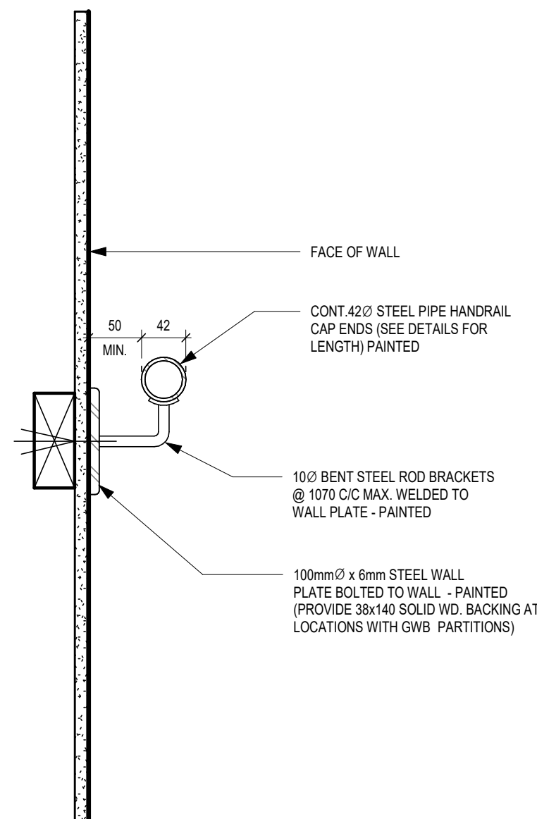
8 A504 WALL MOUNTED HANDRAIL DETAIL 1 : 5
