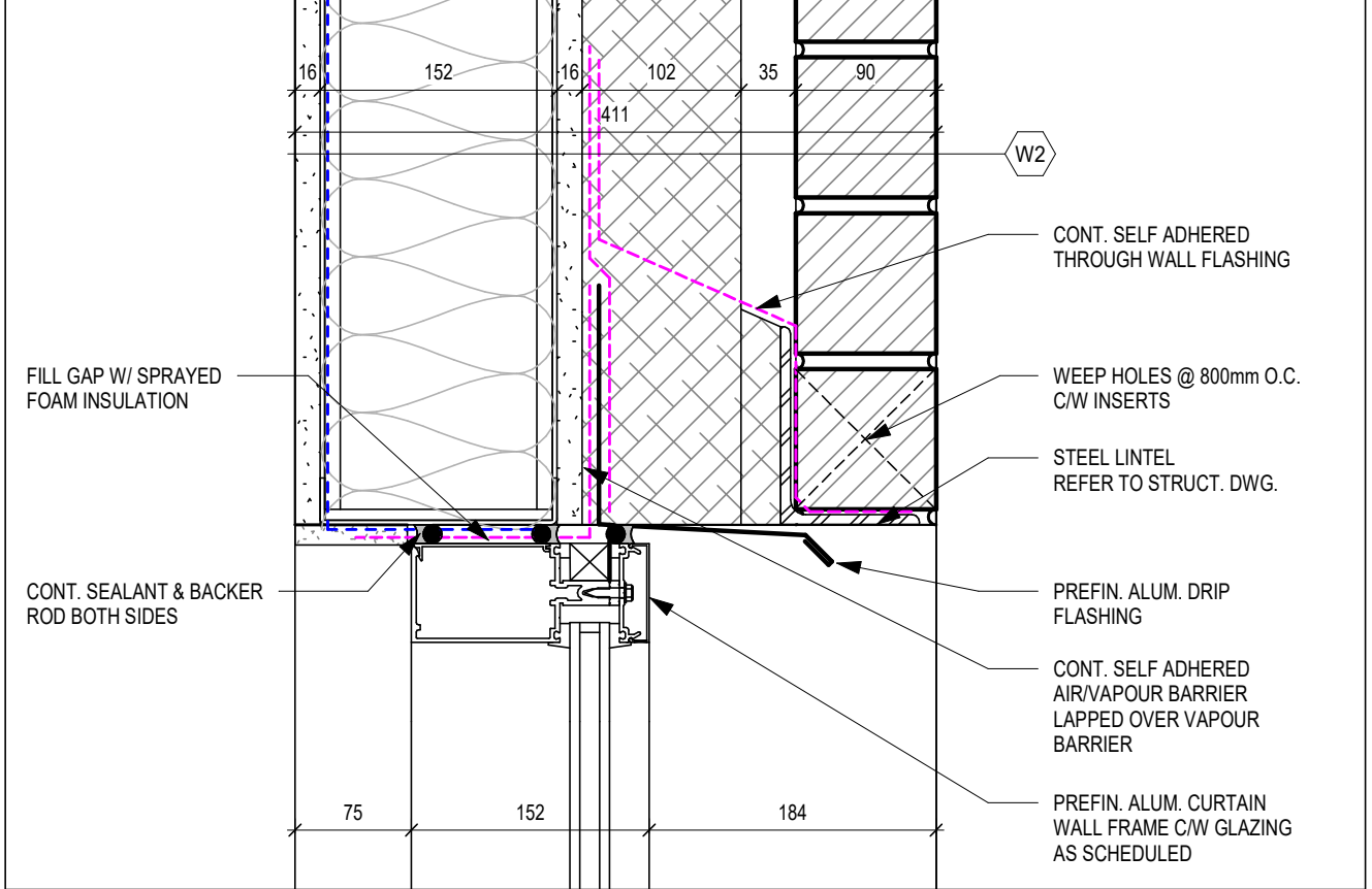
5 SECTION DETAIL A420 1:5
