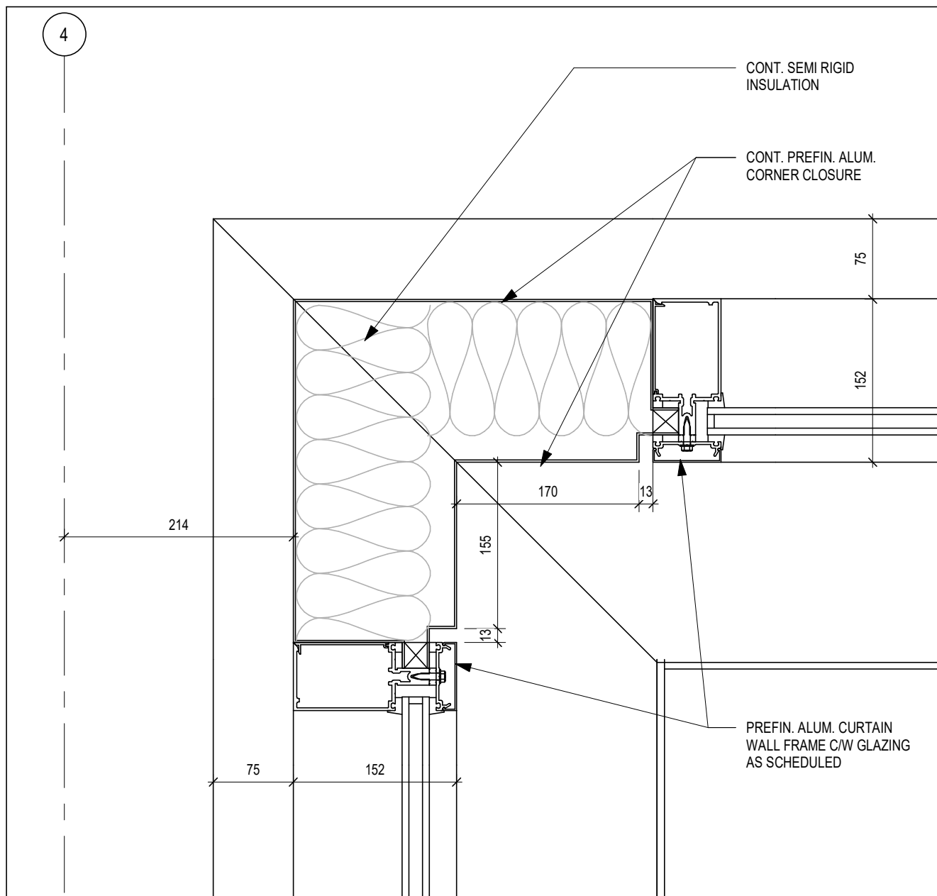
3 A601 PLAN DETAIL 1:5
