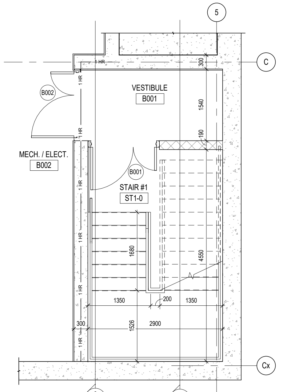
1 STAIR #1 - BASEMENT PLAN A501 1 : 50
