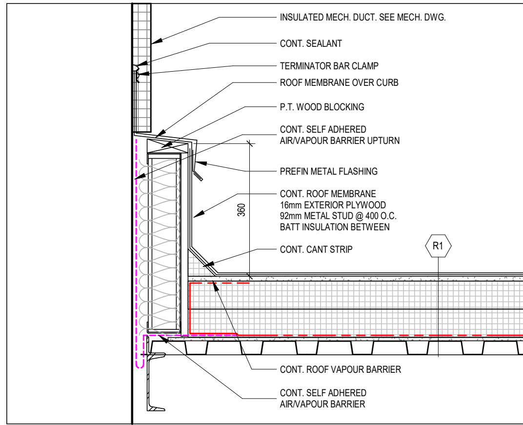
6 TYP. DUCT PENETRATION THRU ROOF DETAIL A206 1 : 10
