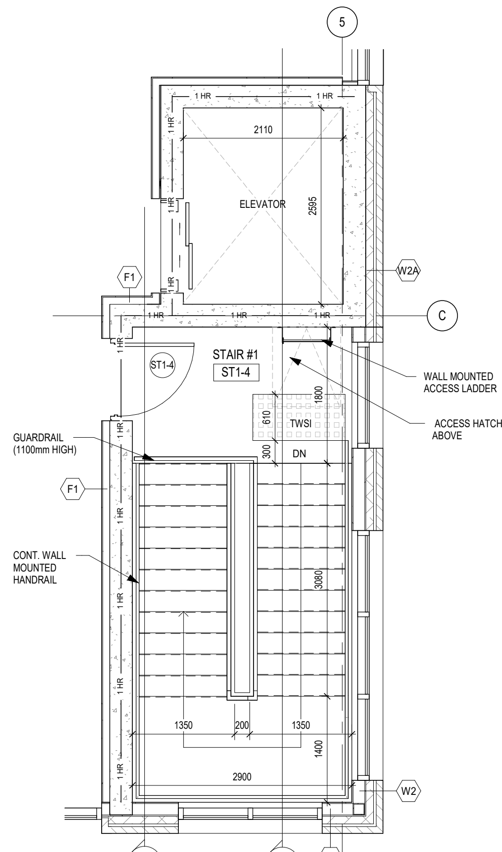
5 STAIR #1 - 4th FLOOR PLAN A501 1 : 50
