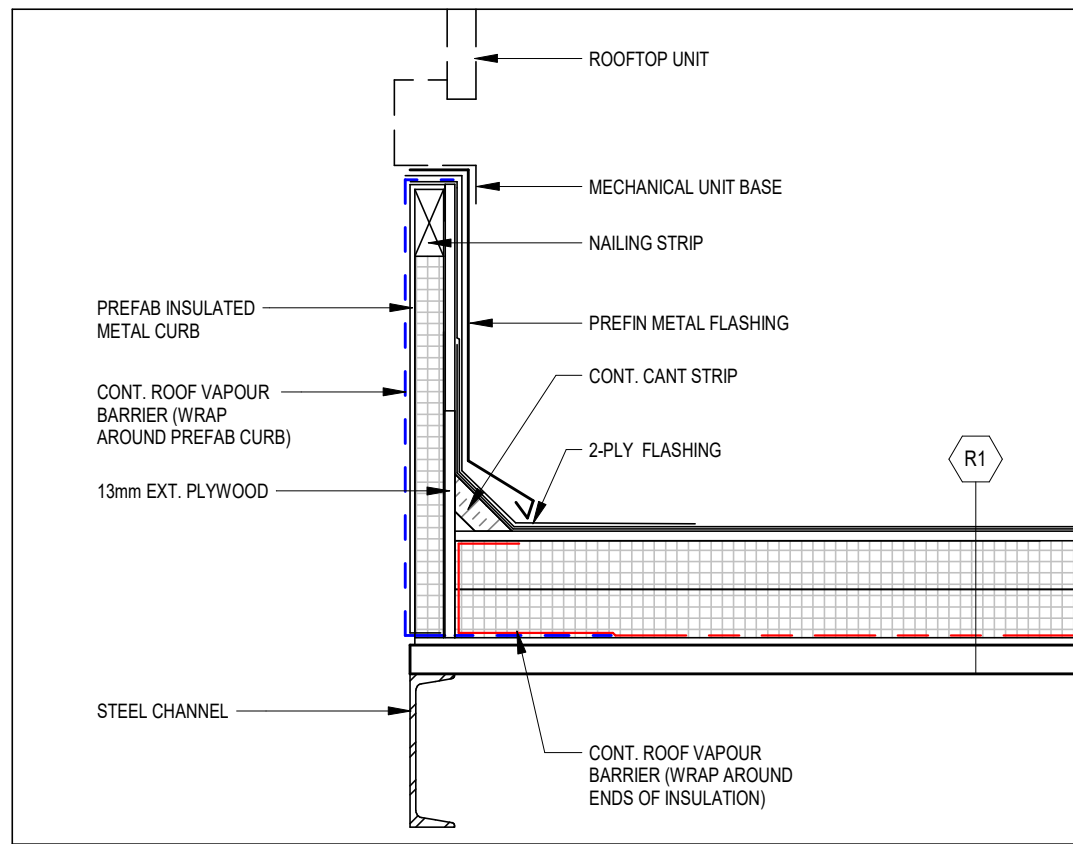
4 TYP. ROOF CURB DETAIL A206 1 : 10
