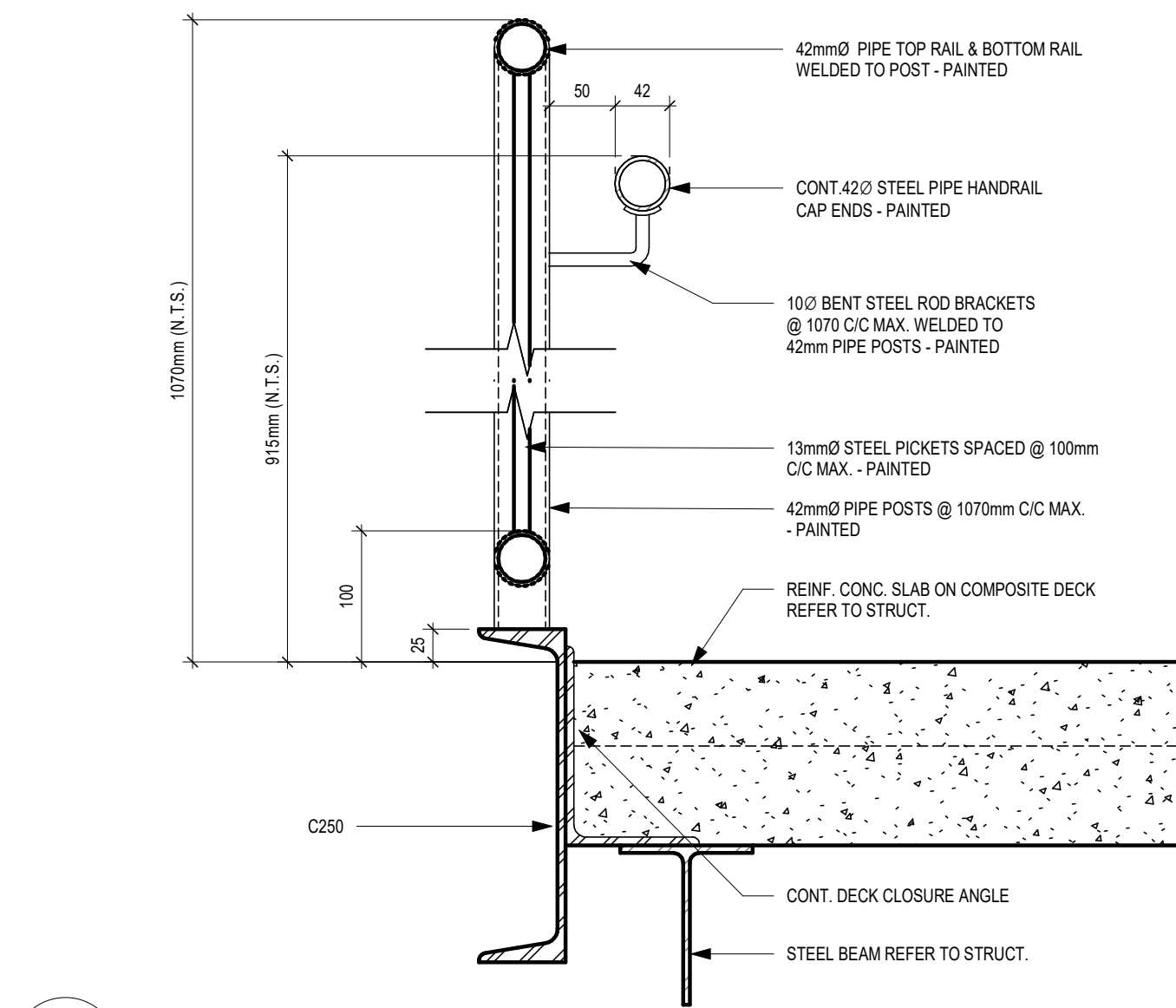
6 A504 TYP. GUARD RAIL DETAIL 1 : 5
