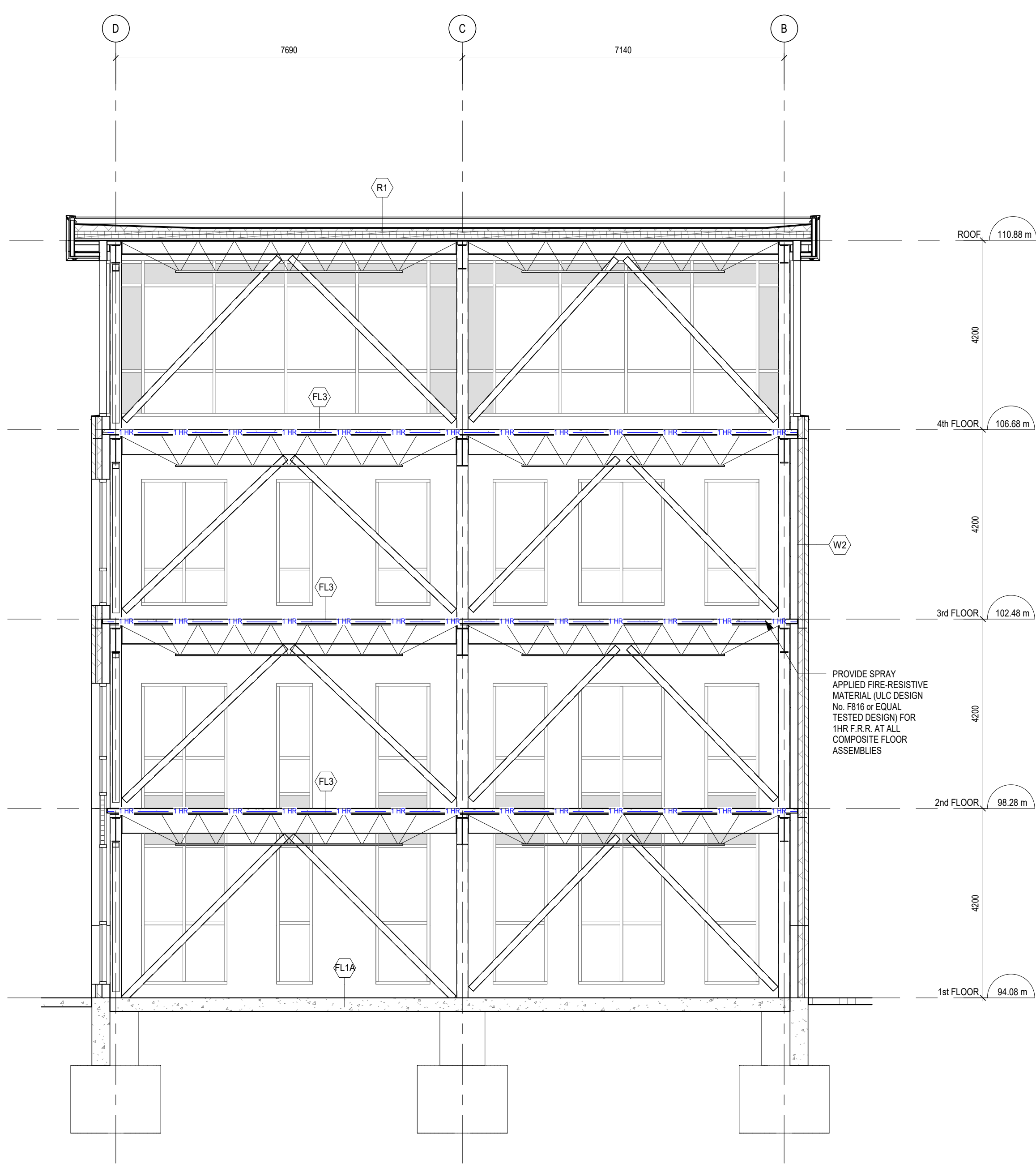
1 A404 BUILDING SECTION 1 : 75
