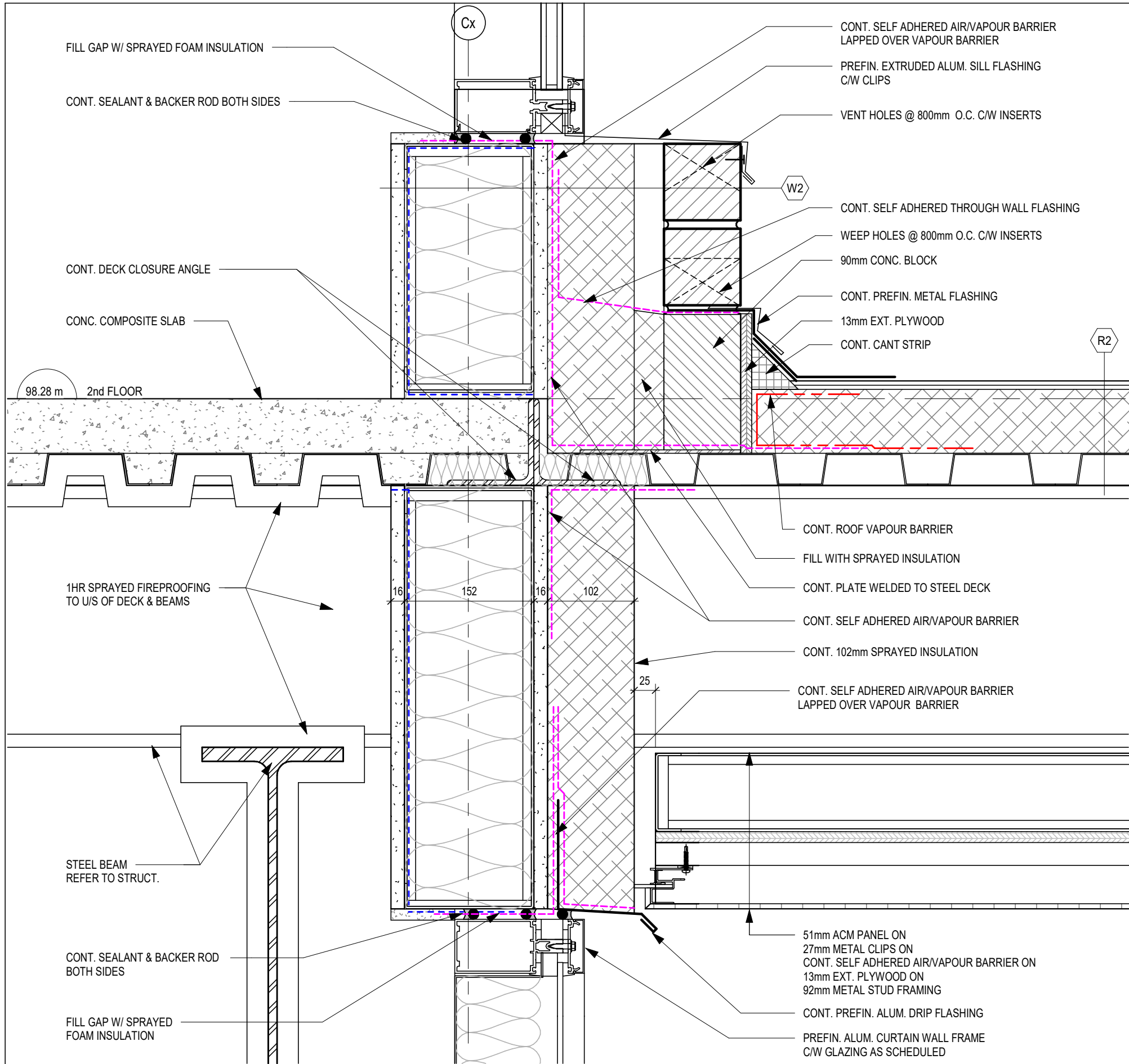
5 SECTION DETAIL A421 1:5
