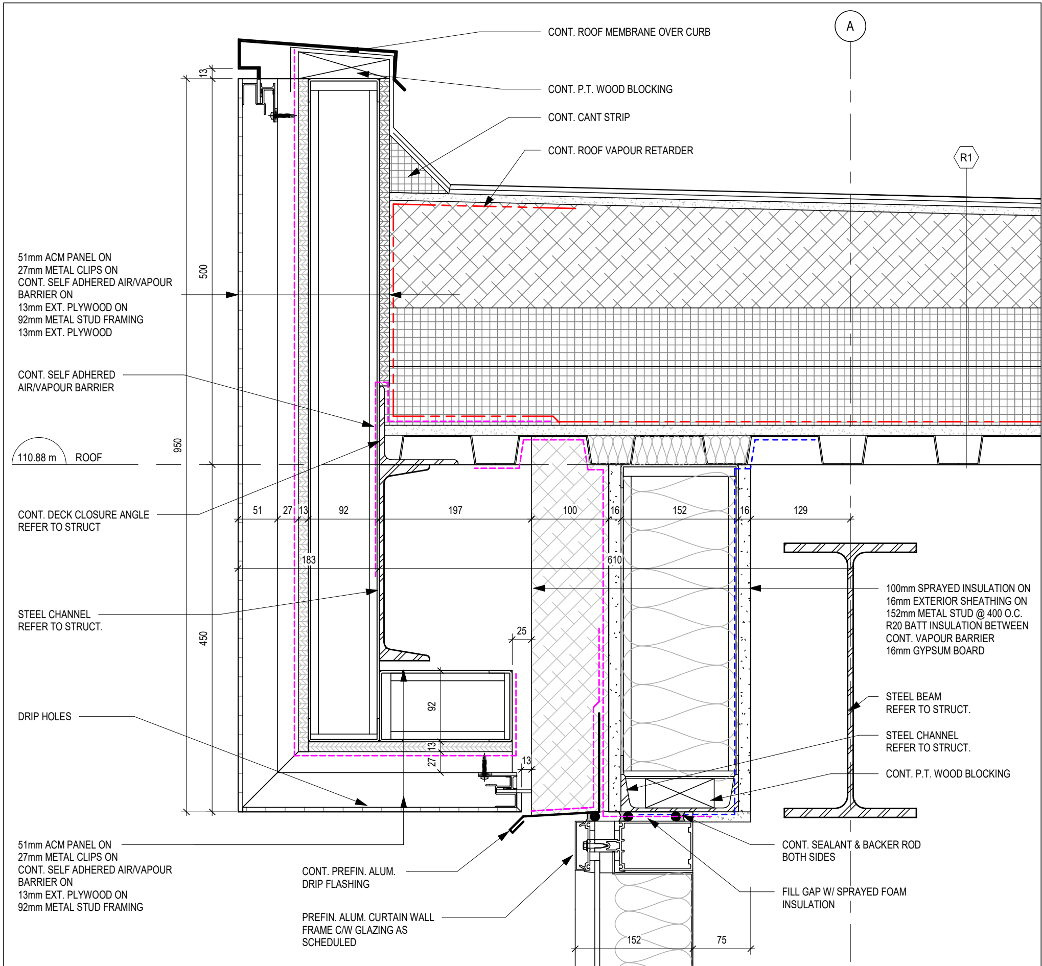
3 SECTION DETAIL A421 1:5
