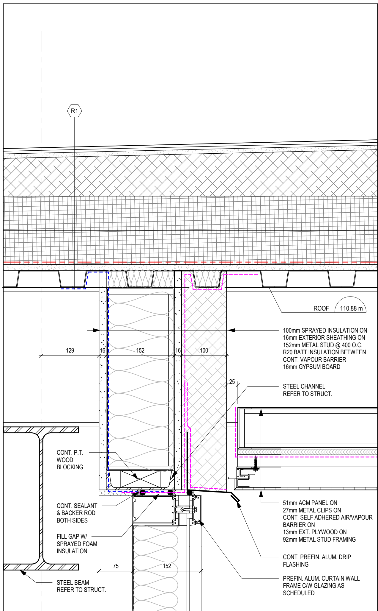
2 SECTION DETAIL A421 1:5
