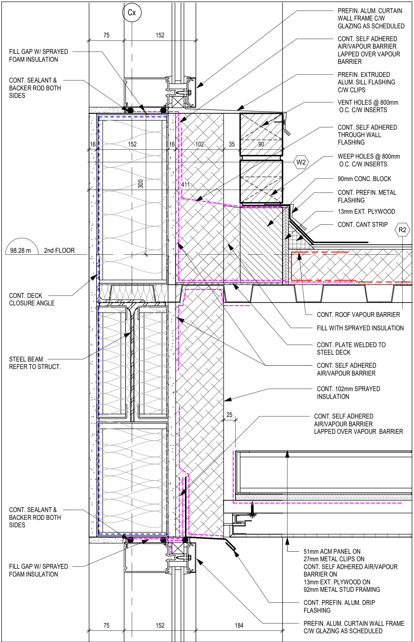
6 SECTION DETAIL A420 1:5
