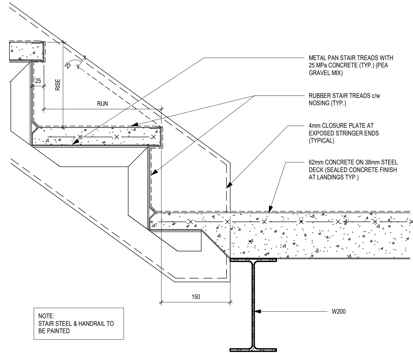
3 A504 TYP. STAIR DETAIL STEEL W/ CONC (BOT LANDING) 1 : 5
