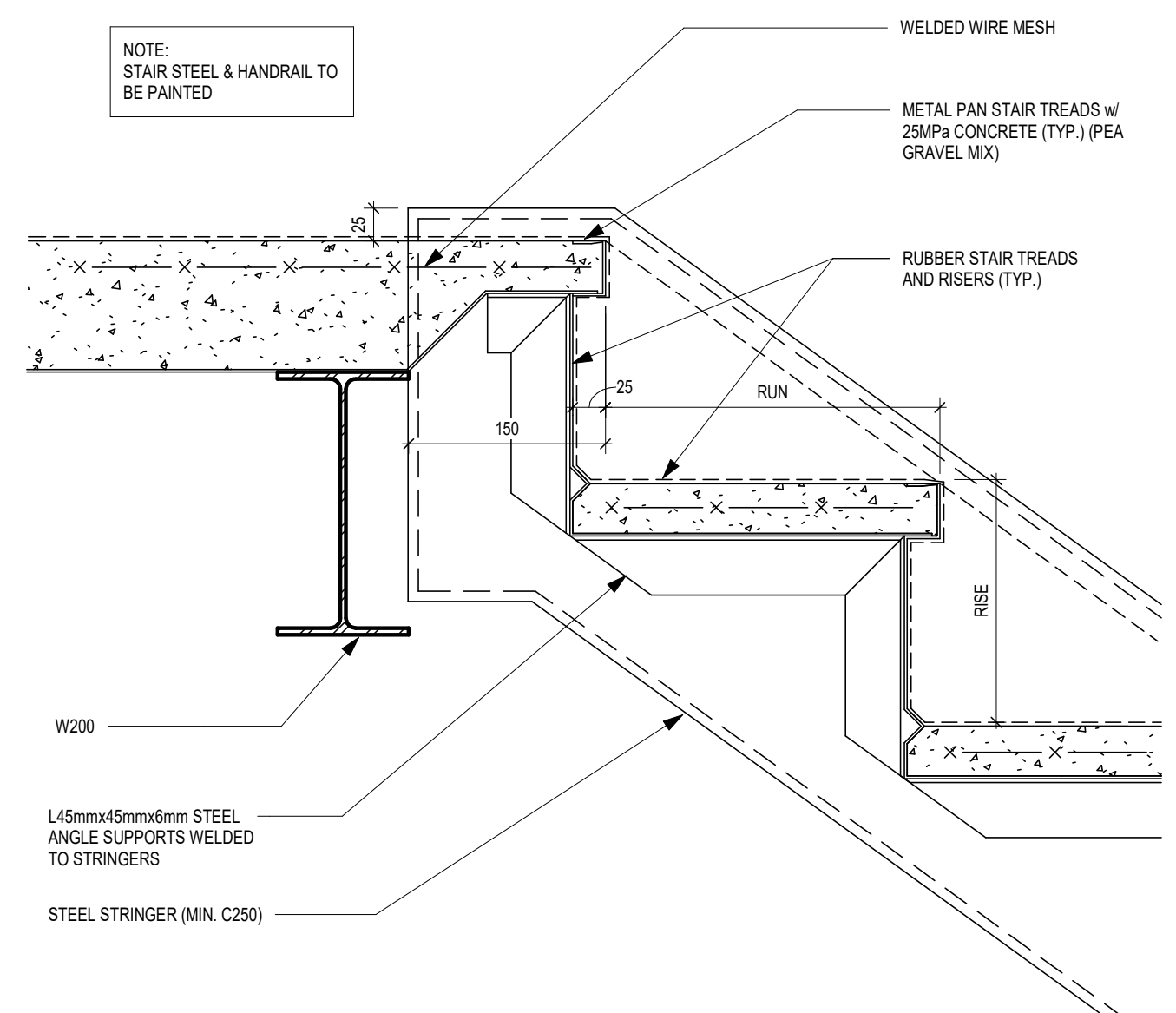
2 A504 TYP. STAIR DETAIL STEEL W/ CONC (TOP LANDING) 1 : 5
