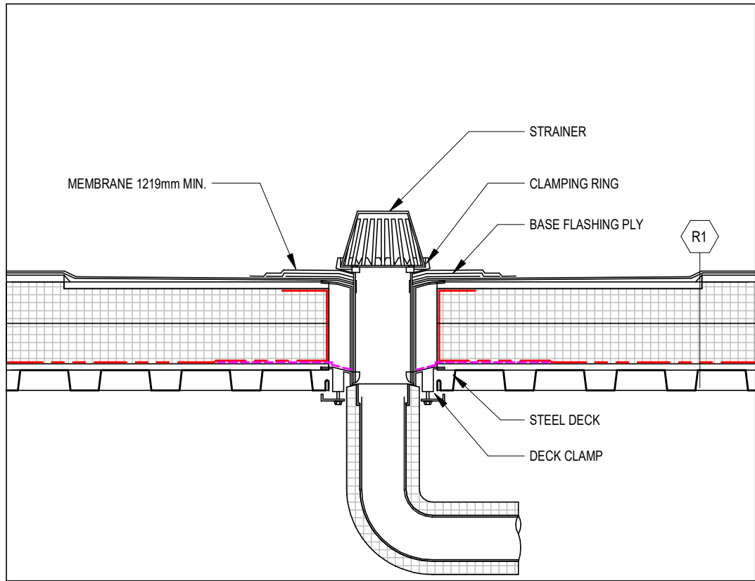
3 TYP. ROOF DRAIN DETAIL A206 1 : 10
