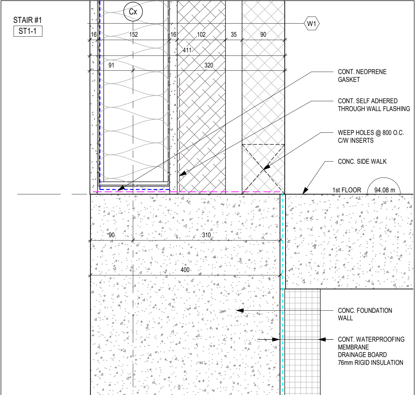
1 SECTION DETAIL A420 1:5
