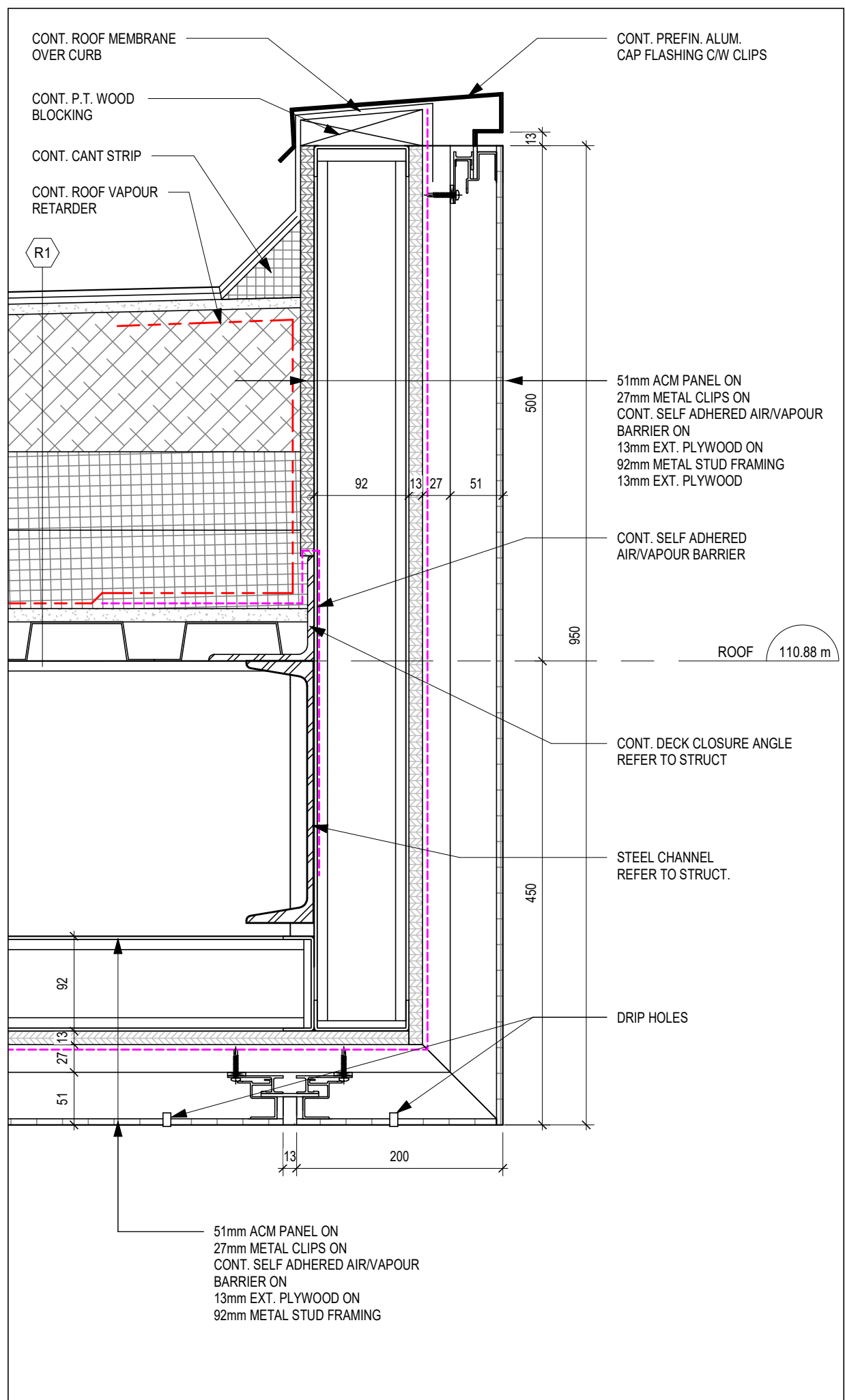
1 SECTION DETAIL A421 1:5
