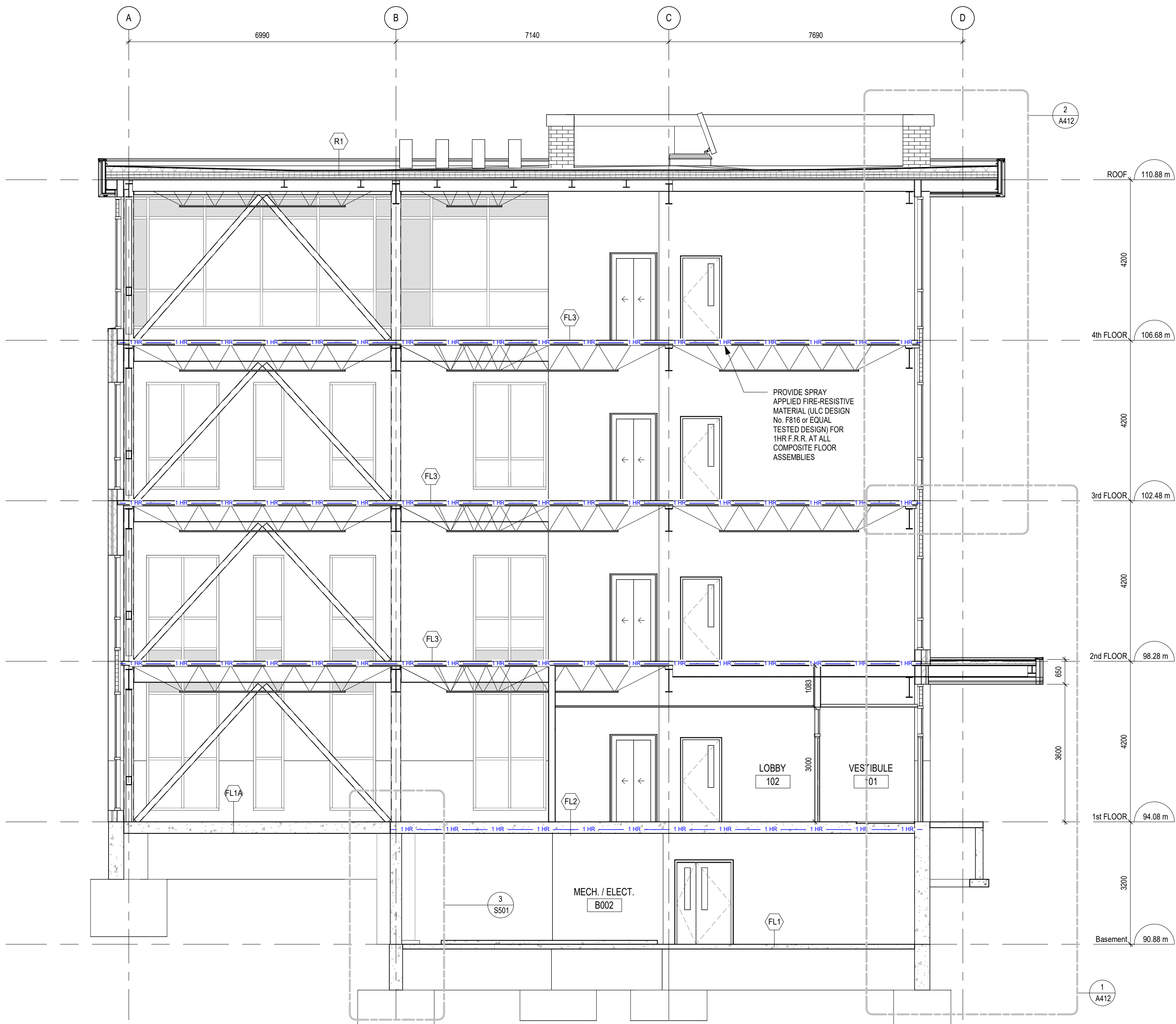
1 A403 BUILDING SECTION 1 : 75
