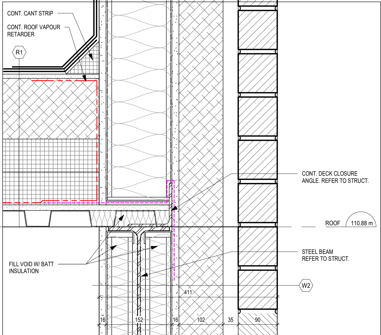
7 SECTION DETAIL A420 1:5
