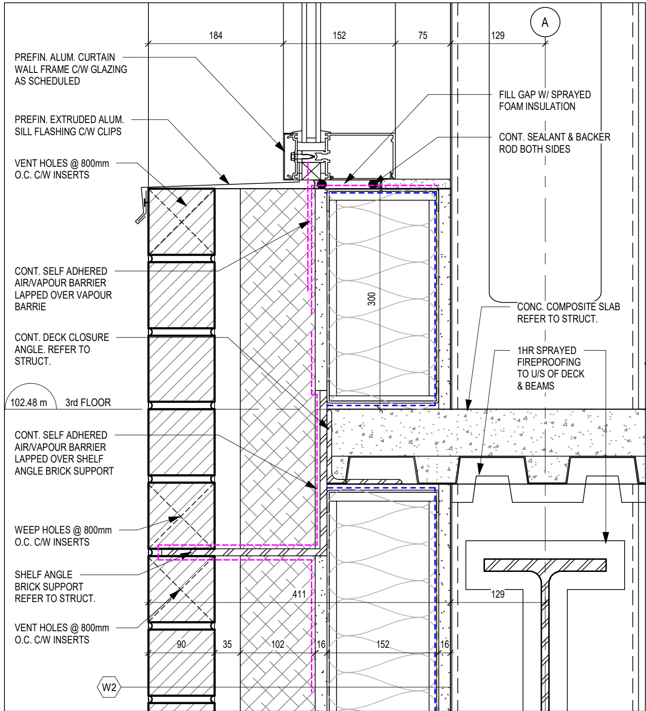
9 SECTION DETAIL A420 1:5
