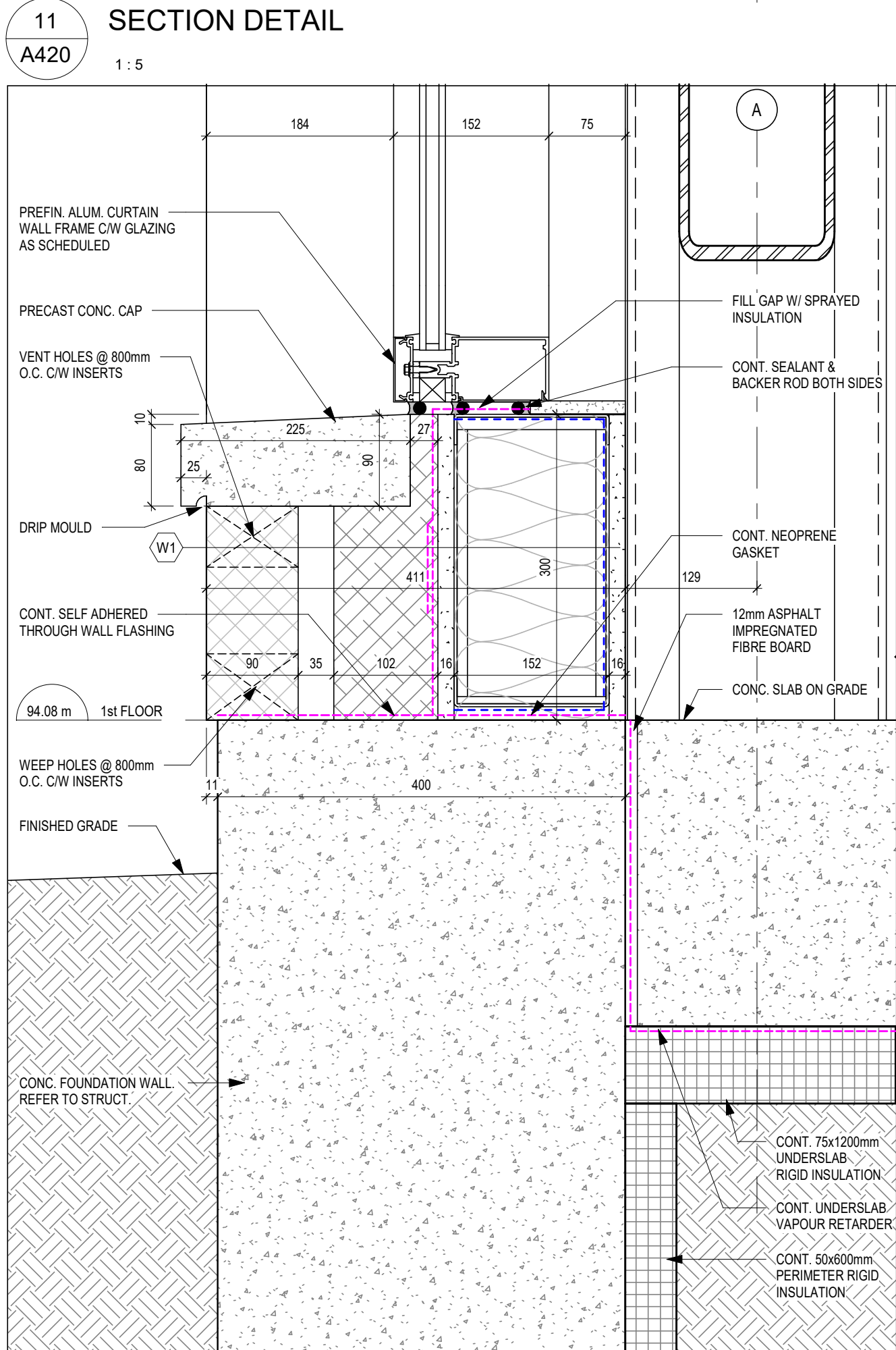
10 SECTION DETAIL A420 1:5
