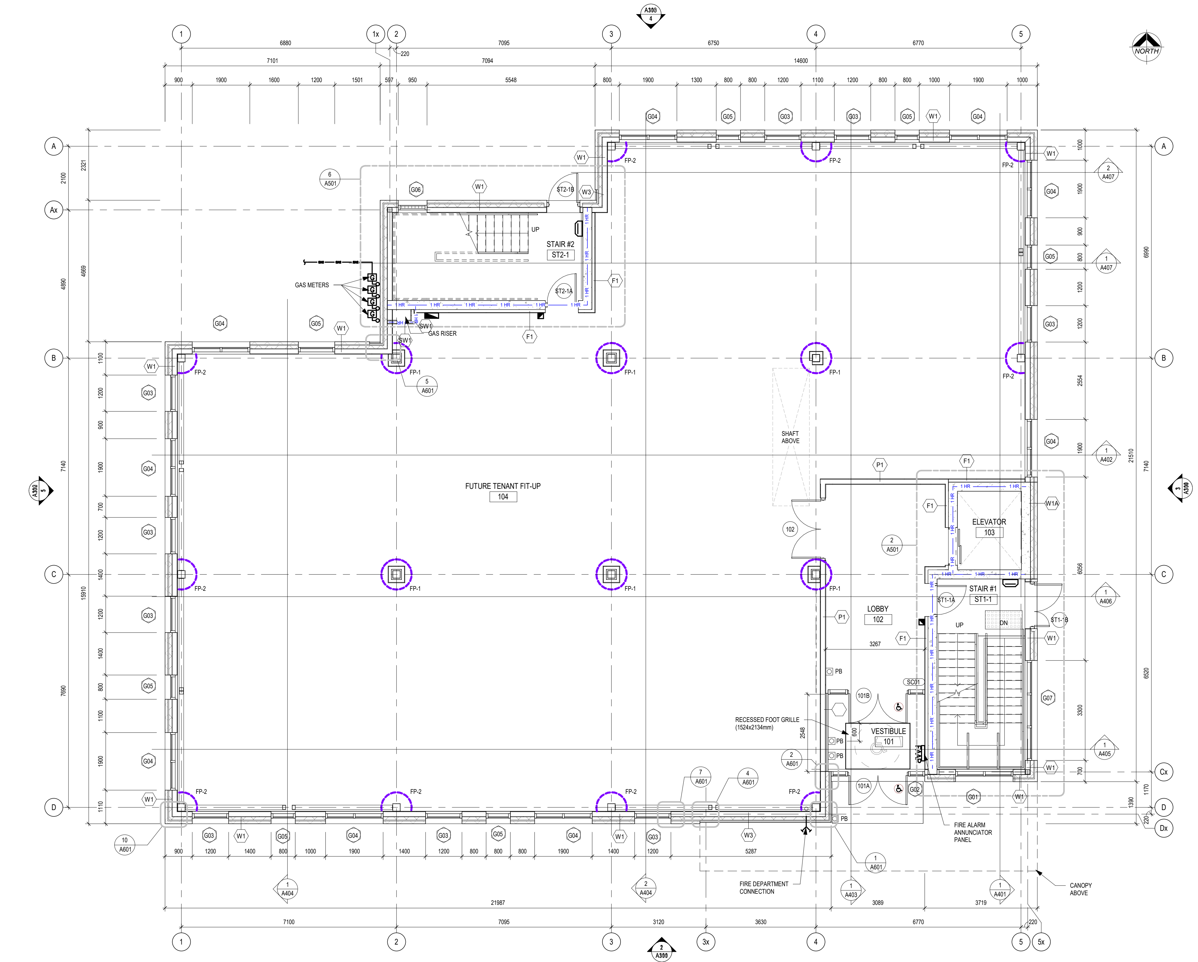
1 A202 1st FLOOR PLAN 1 : 75
