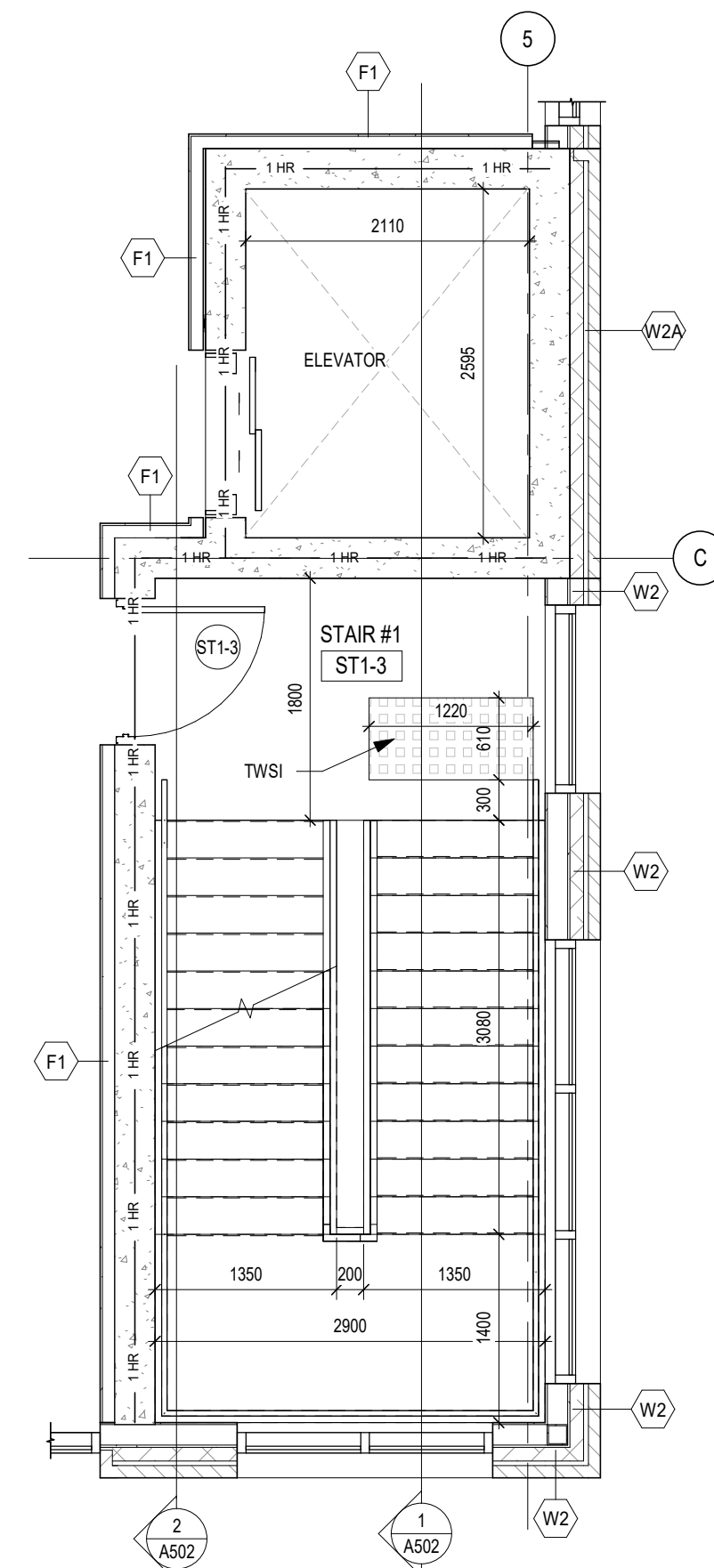
4 STAIR #1 - 3rd FLOOR PLAN A501 1 : 50
