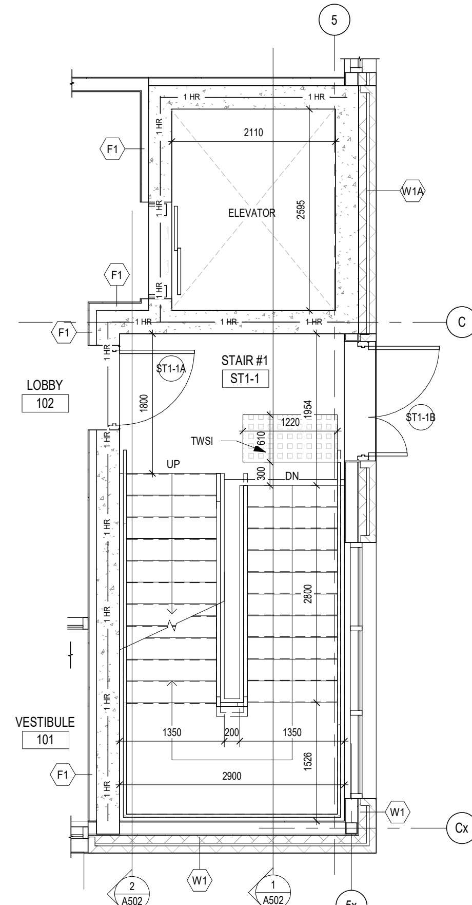
2 STAIR #1 - 1st FLOOR PLAN A501 1 : 50
