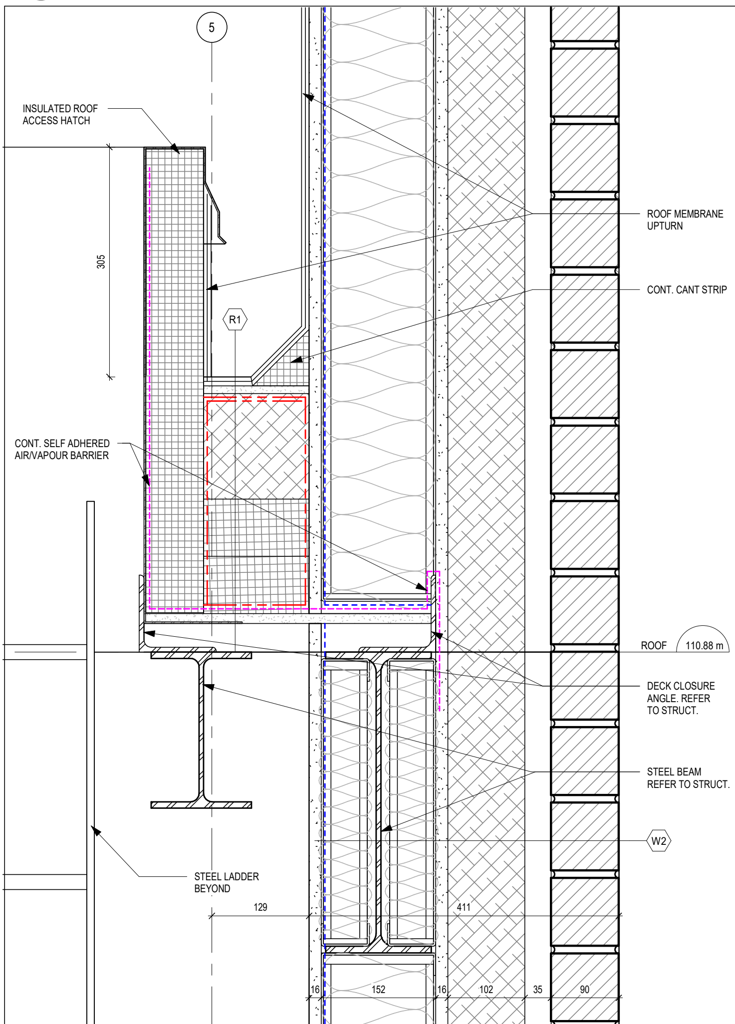
4 SECTION DETAIL A421 1:5
