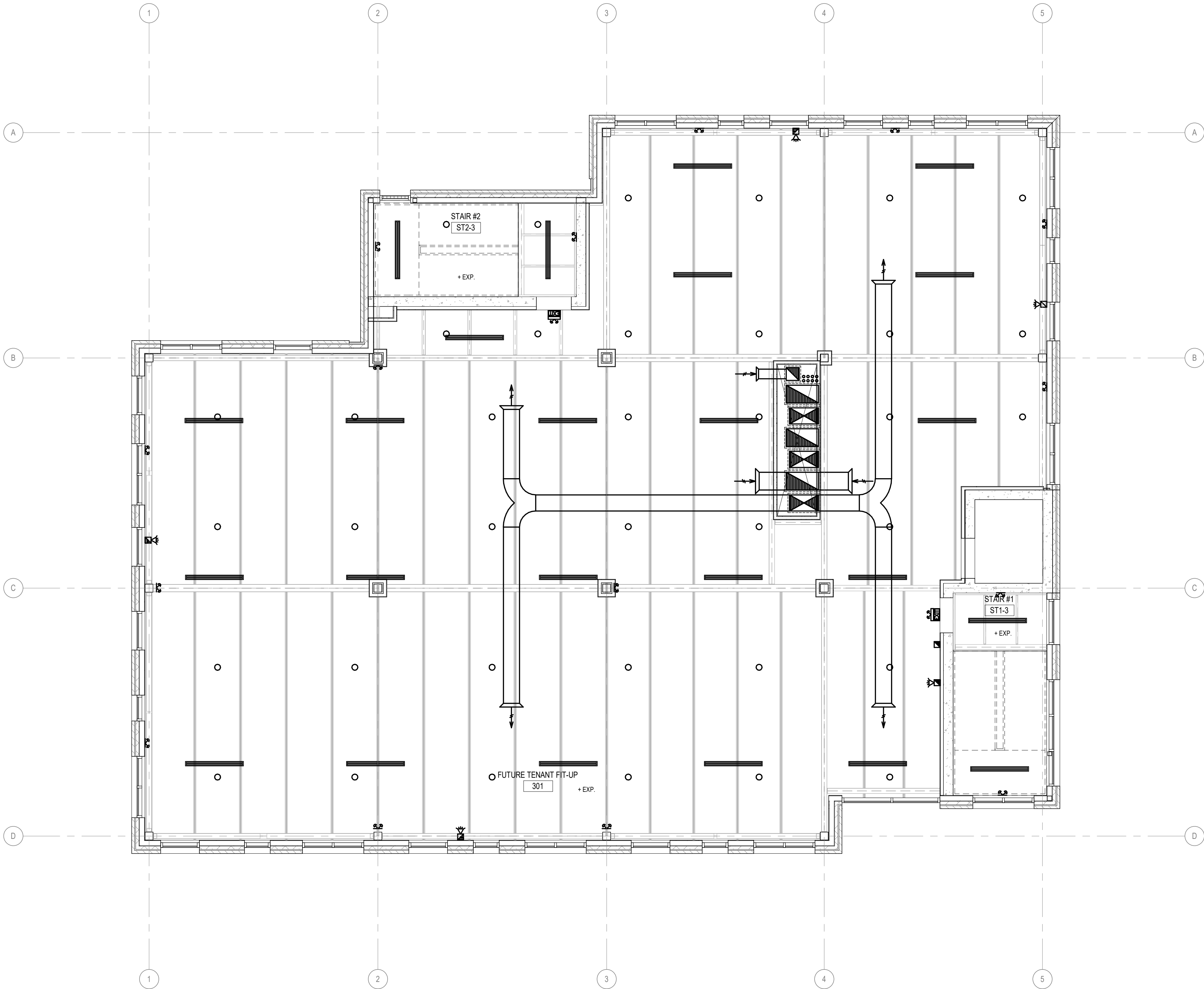
1 A209 3rd FLOOR REFLECTED CEILING PLAN 1 : 75
