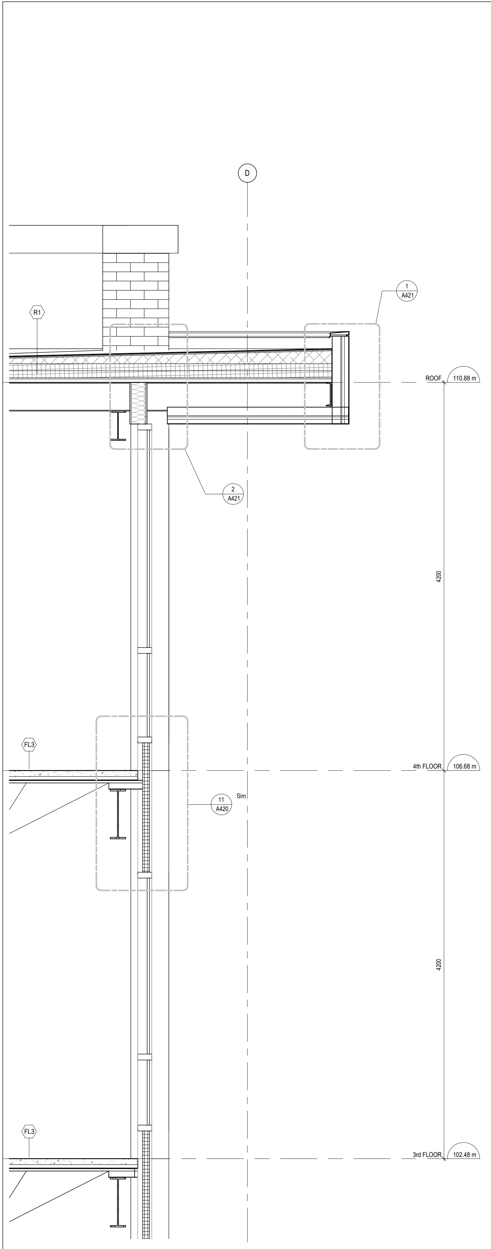
2 WALL SECTION A412 1:25
