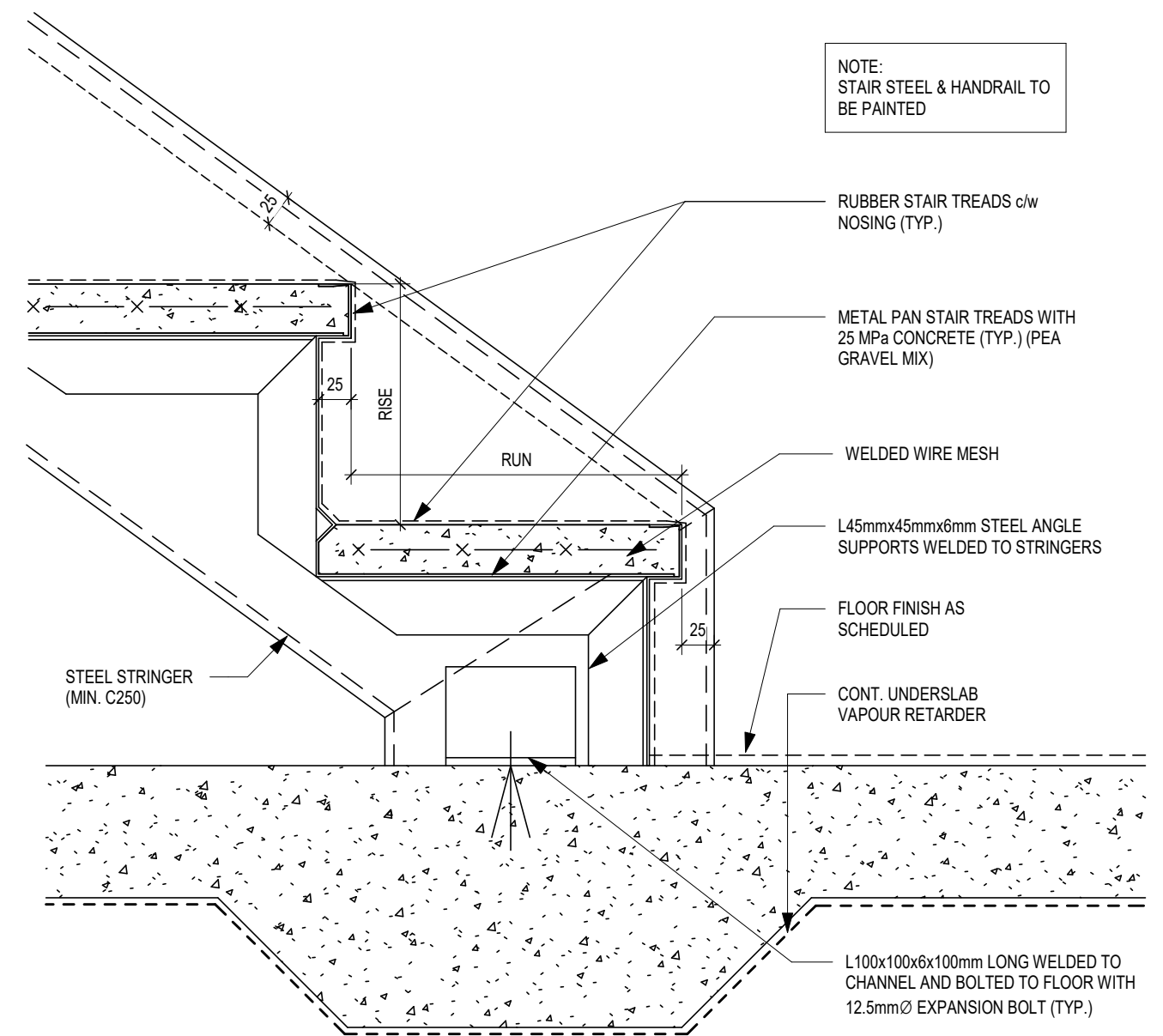
1 A504 TYP. STAIR DETAIL STEEL W/ CONC (BOT) 1 : 5
