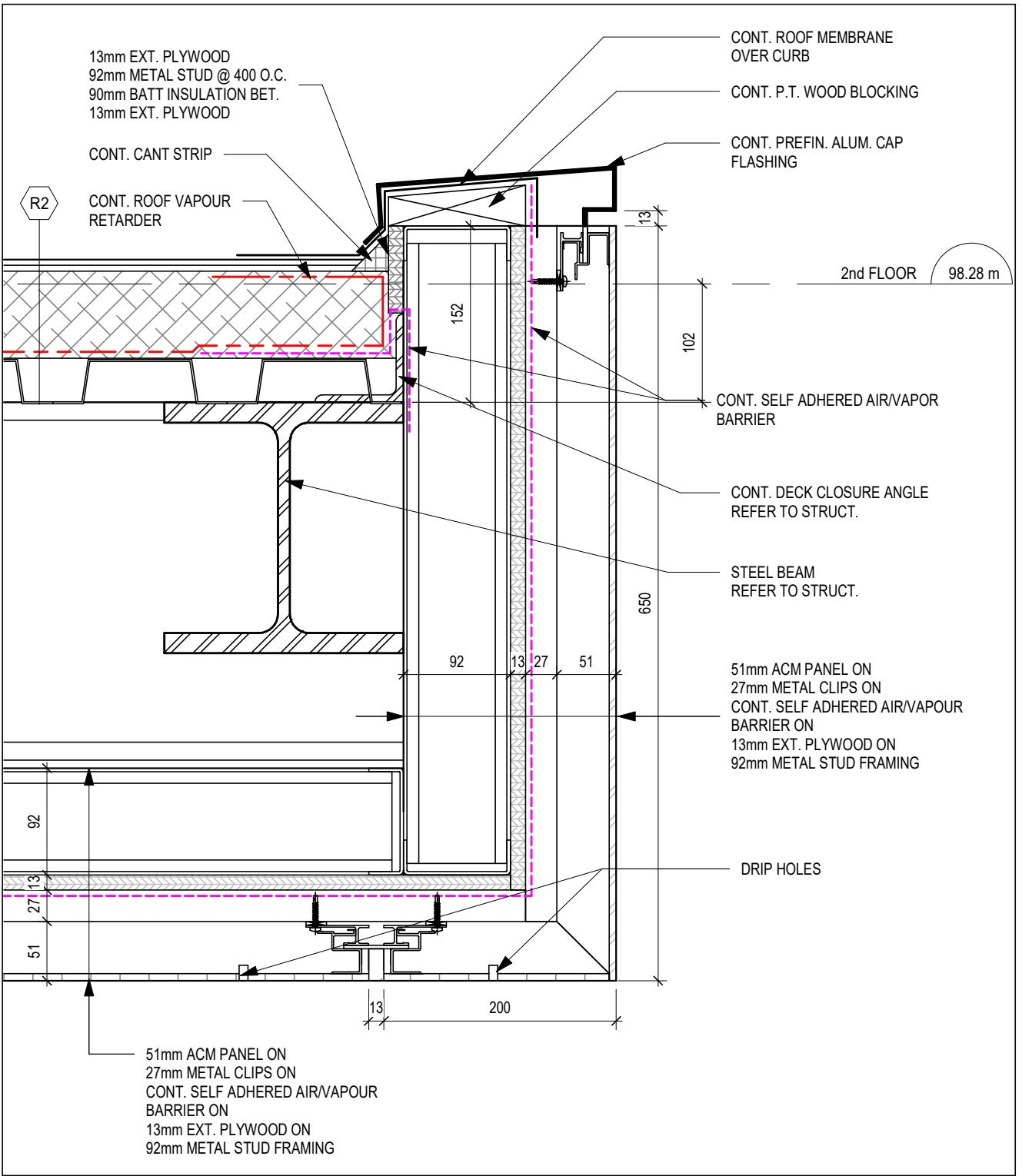
3 SECTION DETAIL A420 1:5
