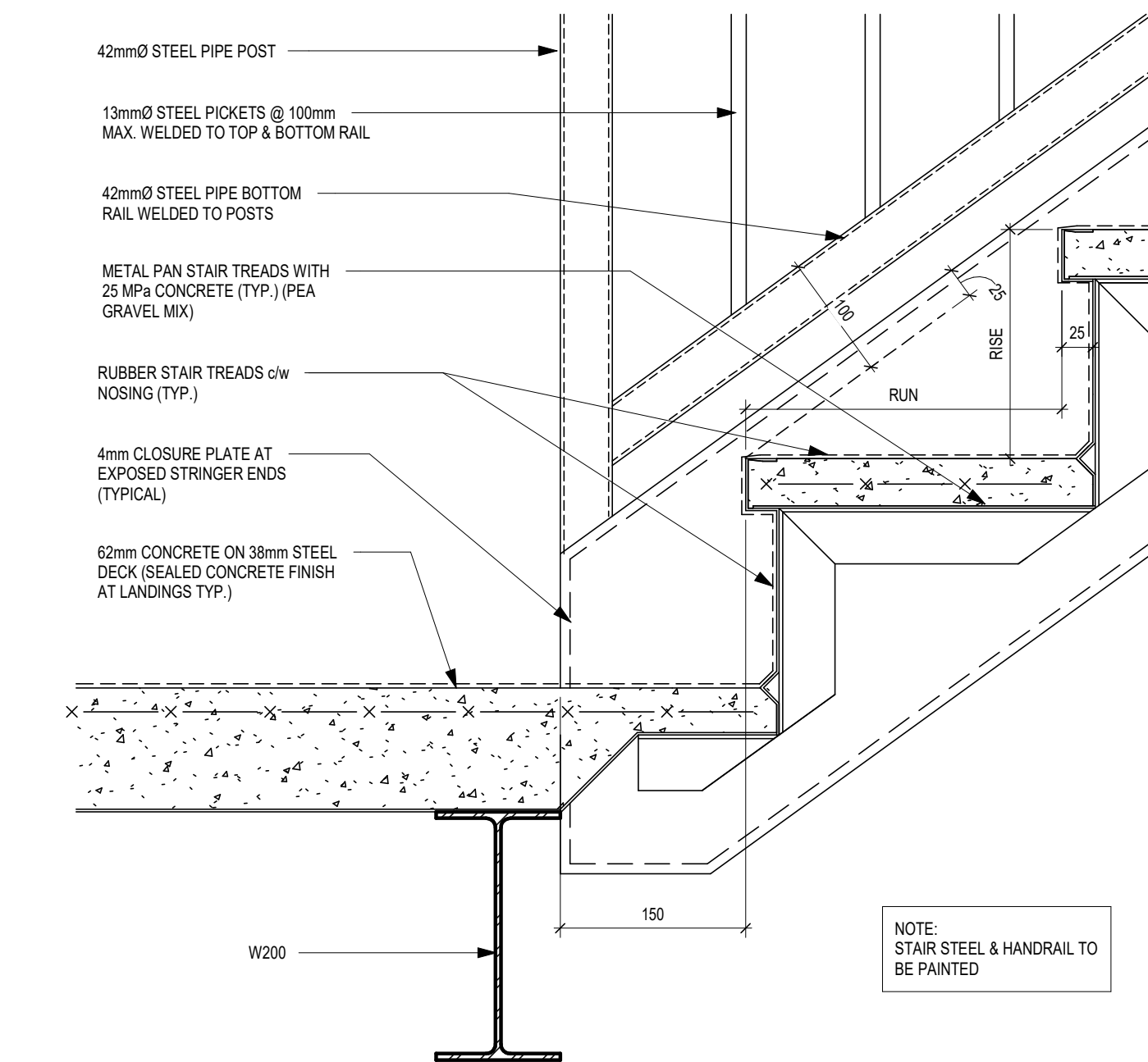
4 A504 TYP. STAIR DETAIL STEEL W/ CONC (BOT LANDING) 1 : 5
