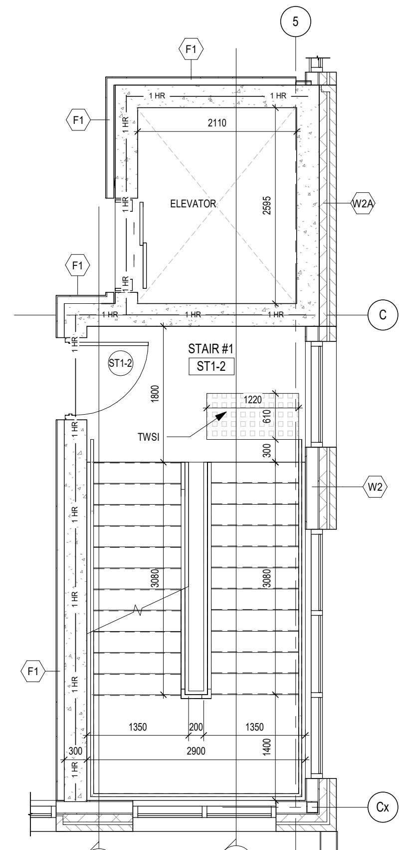
3 STAIR #1 - 2nd FLOOR PLAN A501 1 : 50
