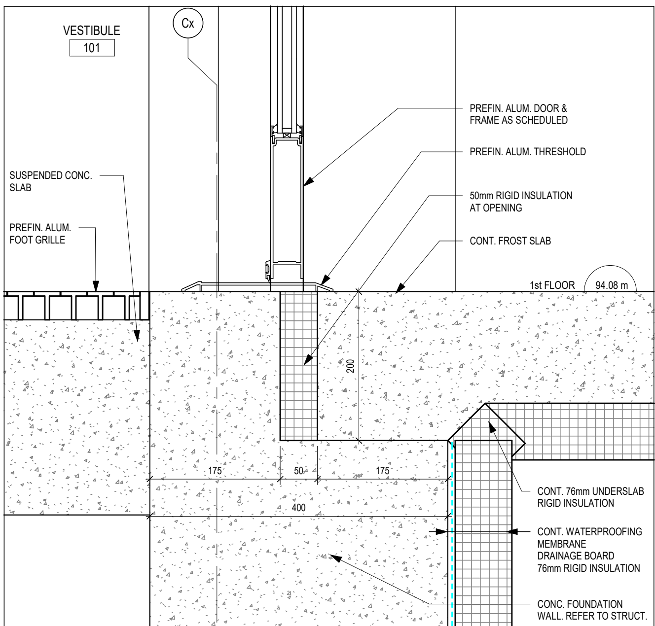
6 SECTION DETAIL A421 1:5
