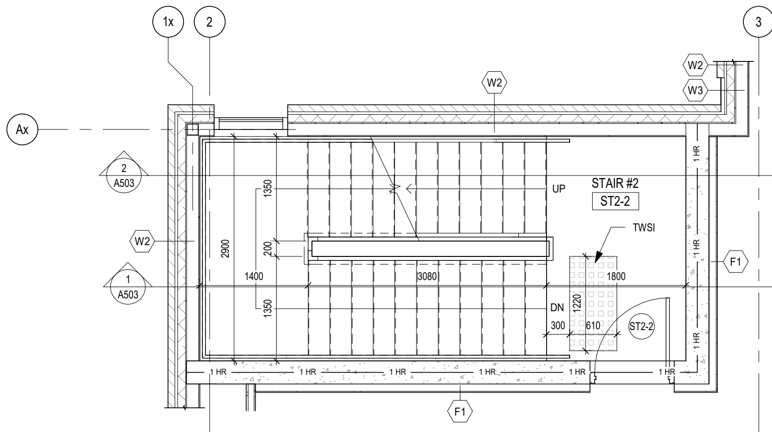
7 STAIR #2 - 2nd FLOOR PLAN A501 1 : 50
