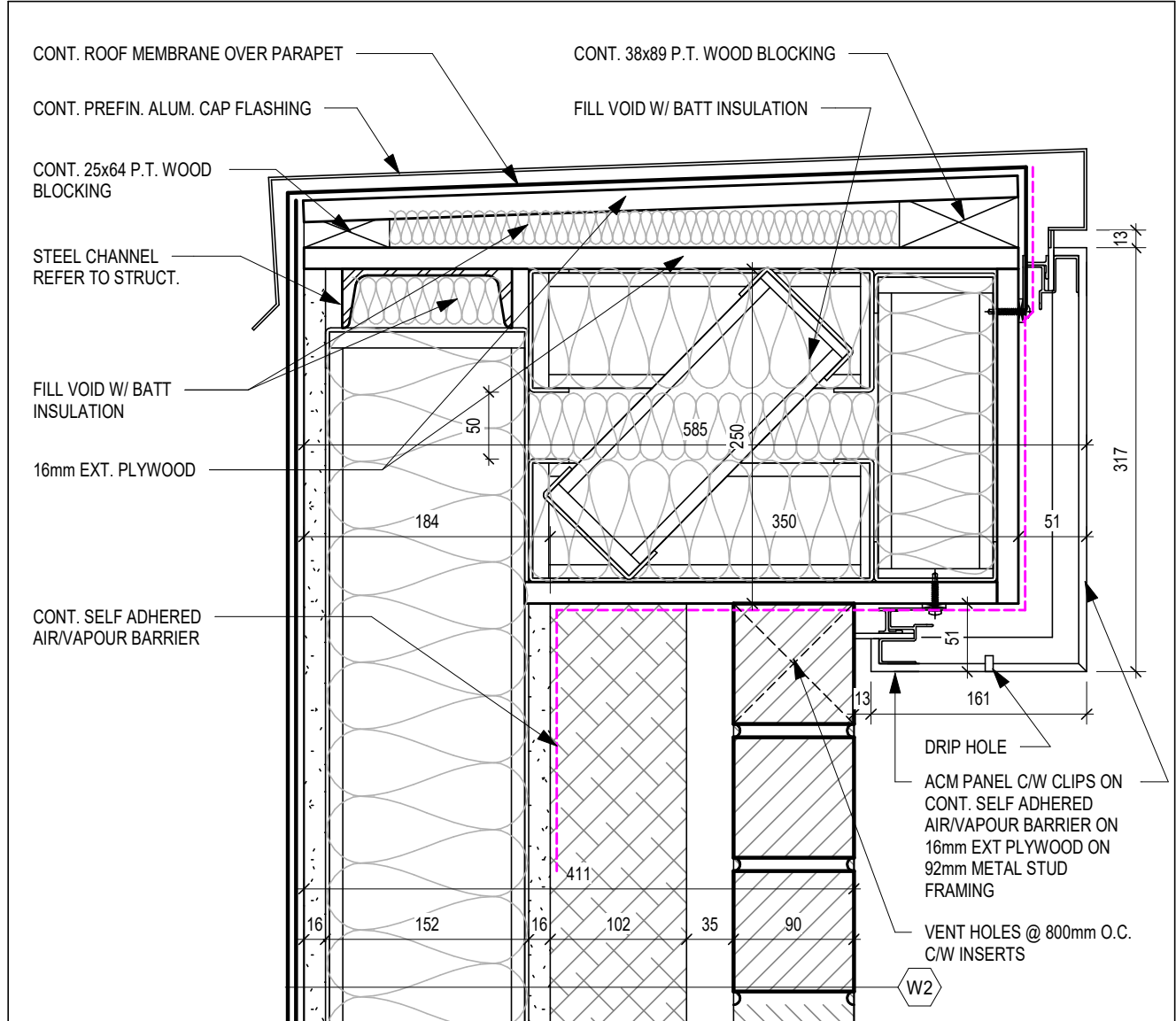
8 SECTION DETAIL A420 1:5
