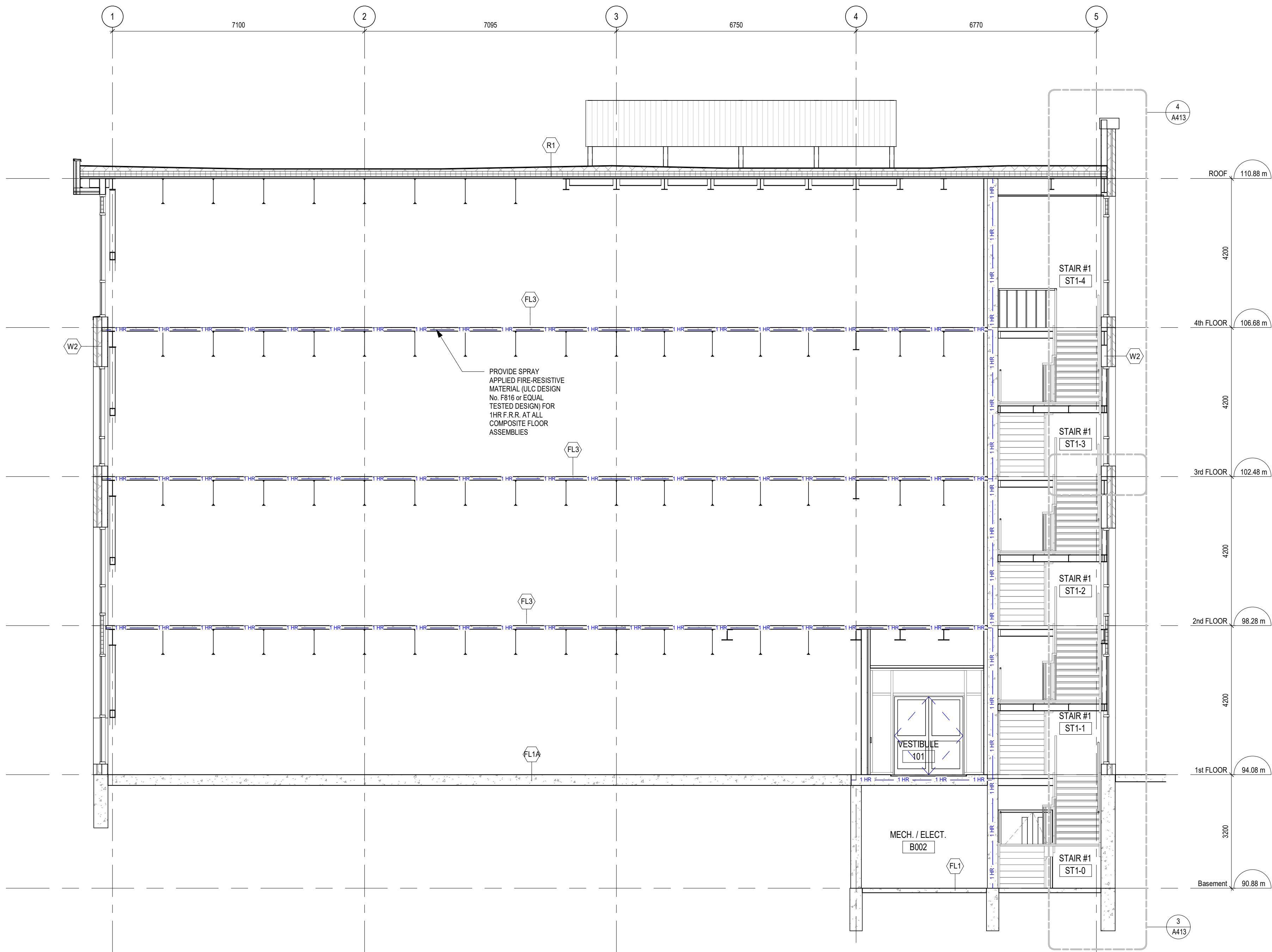
1 BUILDING SECTION A405 1 : 75
