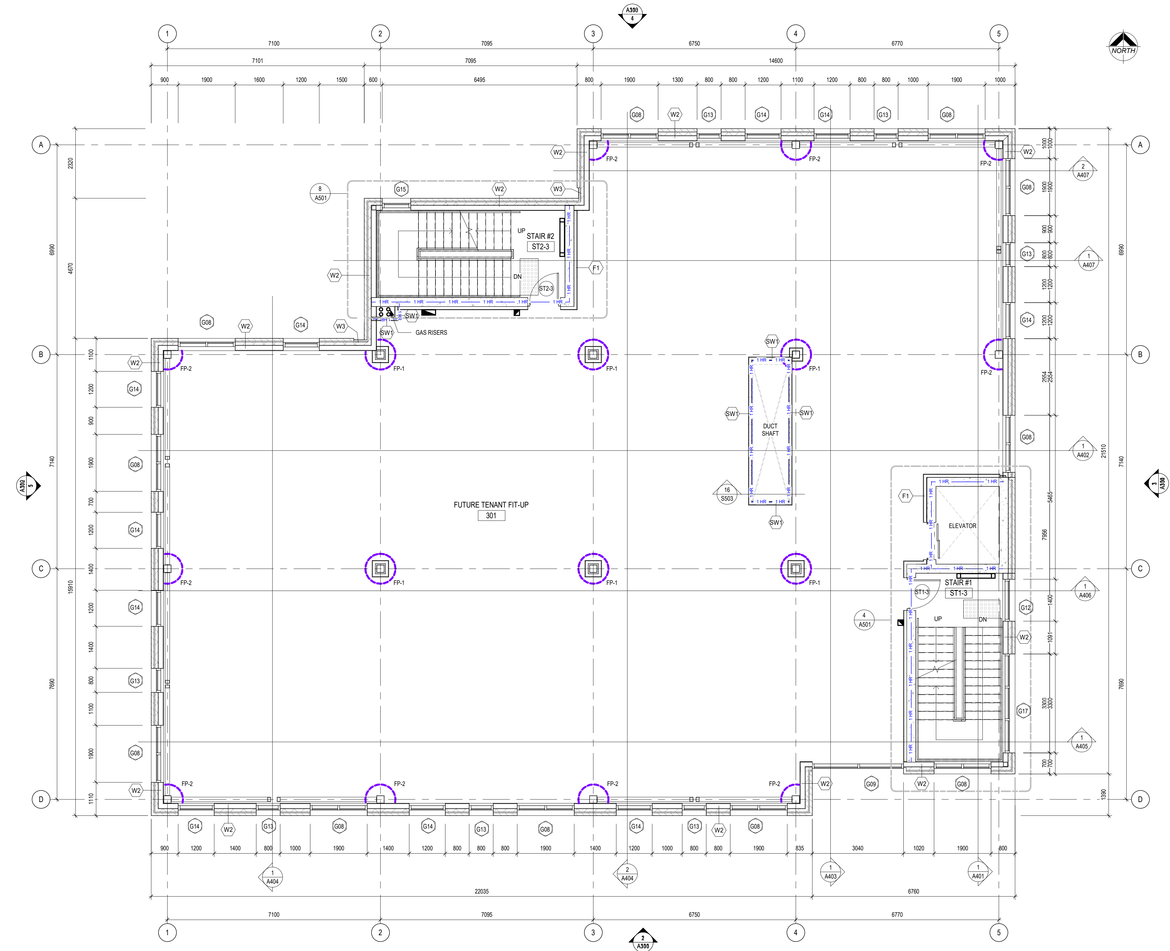
1 A204 3rd FLOOR PLAN 1 : 75
