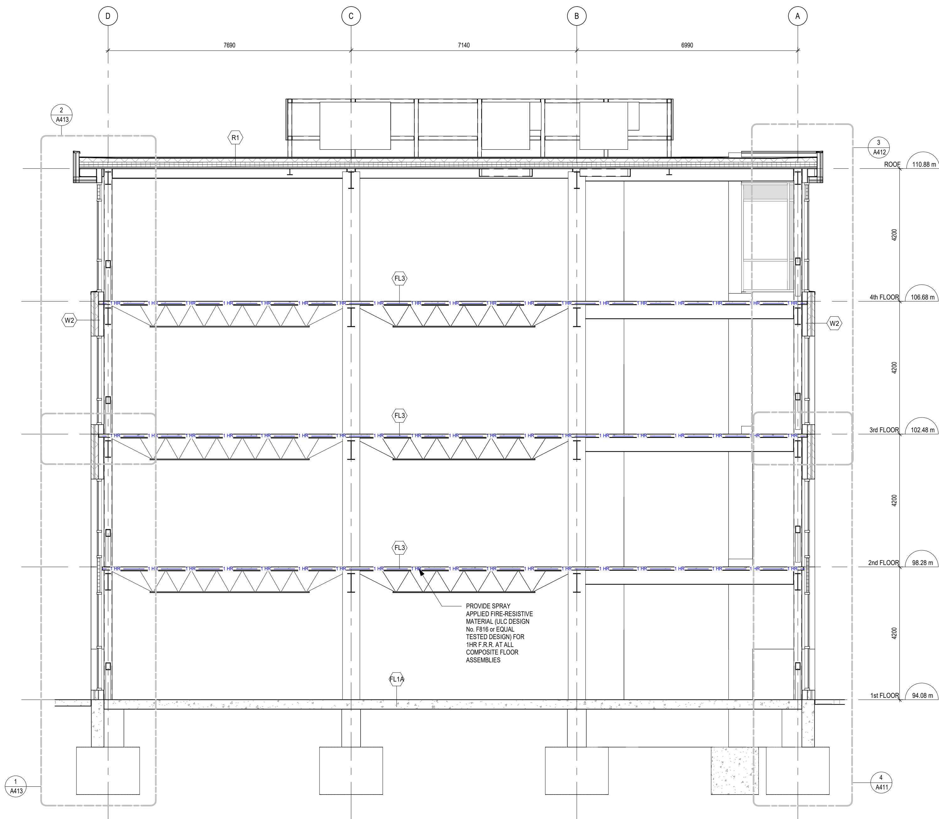
2 A404 BUILDING SECTION 1 : 75
