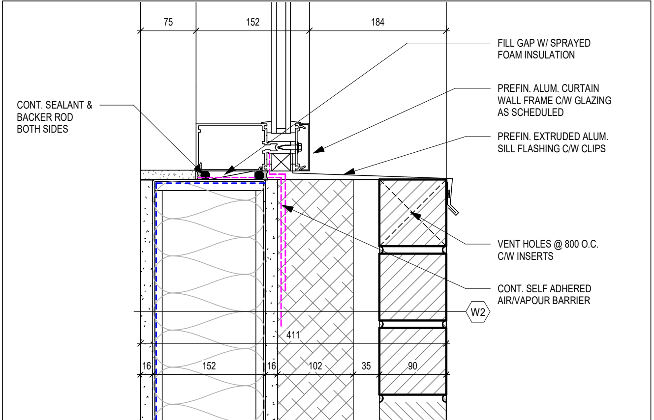
4 SECTION DETAIL A420 1:5
