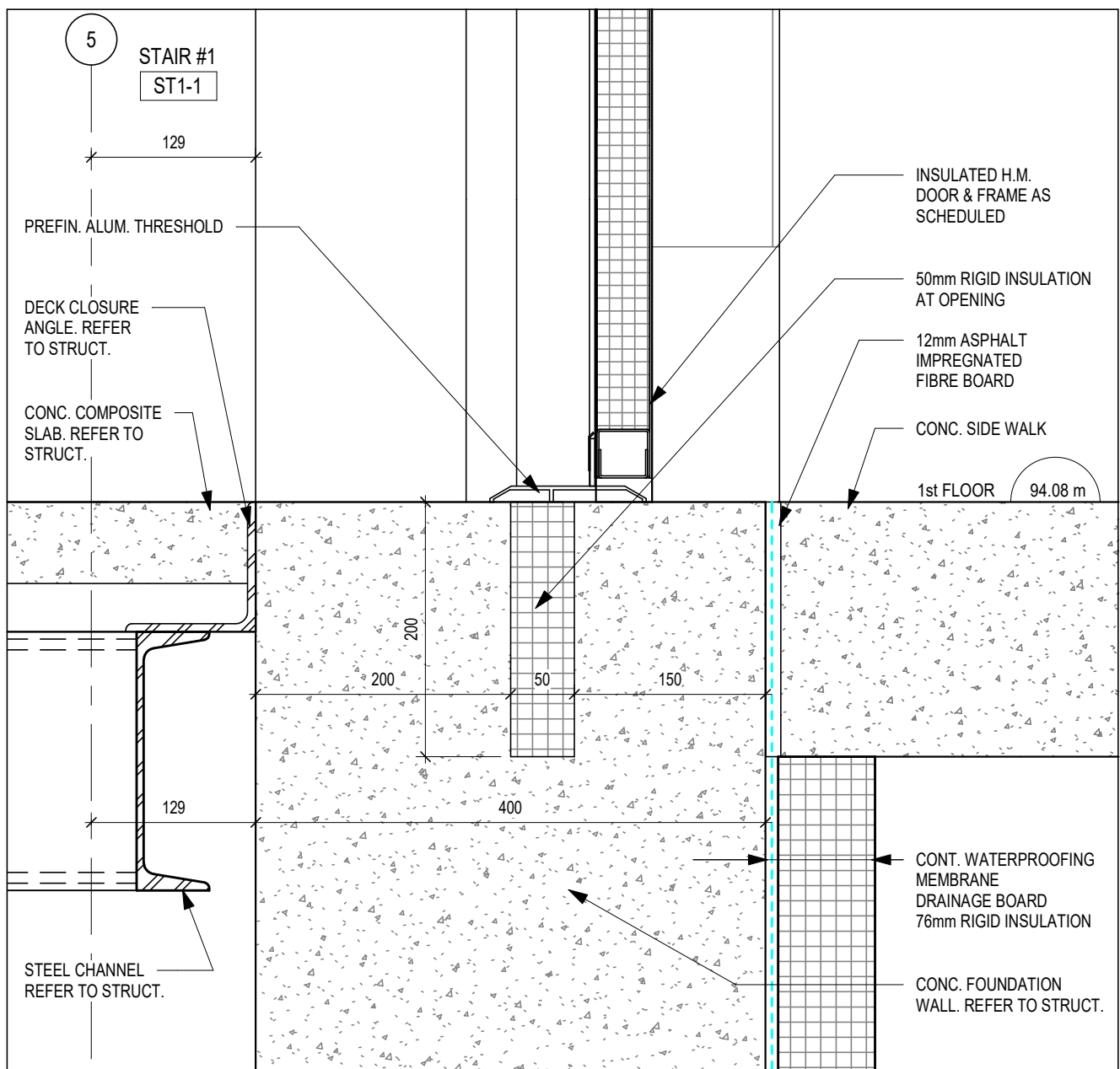
7 SECTION DETAIL A421 1:5
