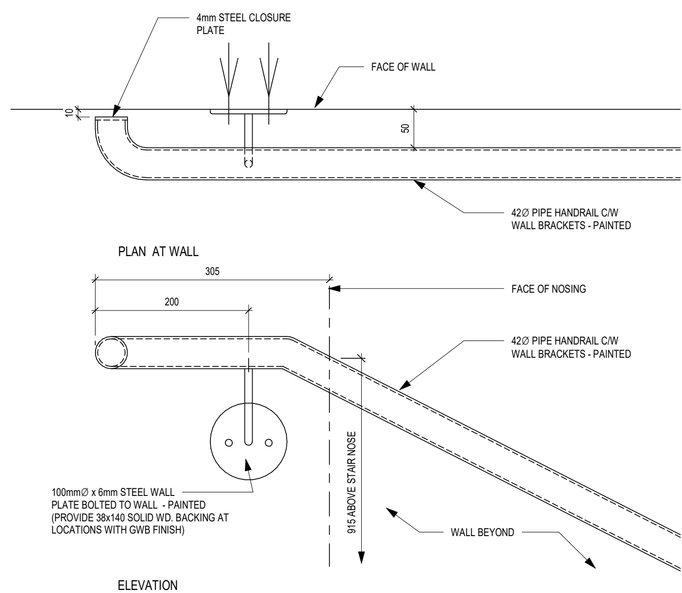
7 A504 WALL MOUNTED HANDRAIL DETAIL 1 : 5
