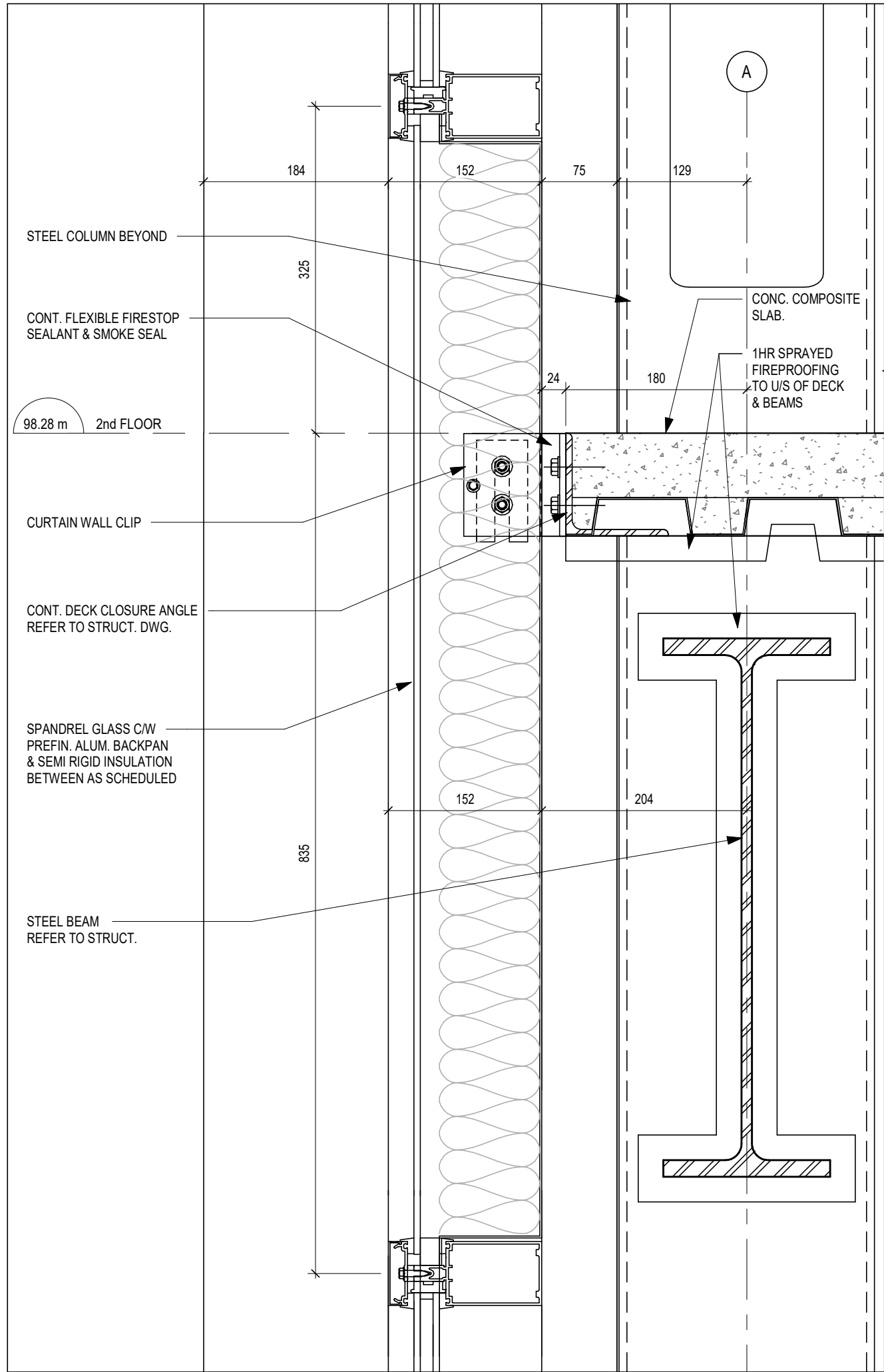
9 SECTION DETAIL A420 1:5
