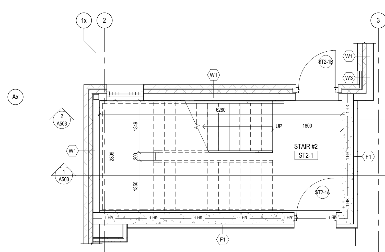
6 STAIR #2 - 1st FLOOR PLAN A501 1 : 50
