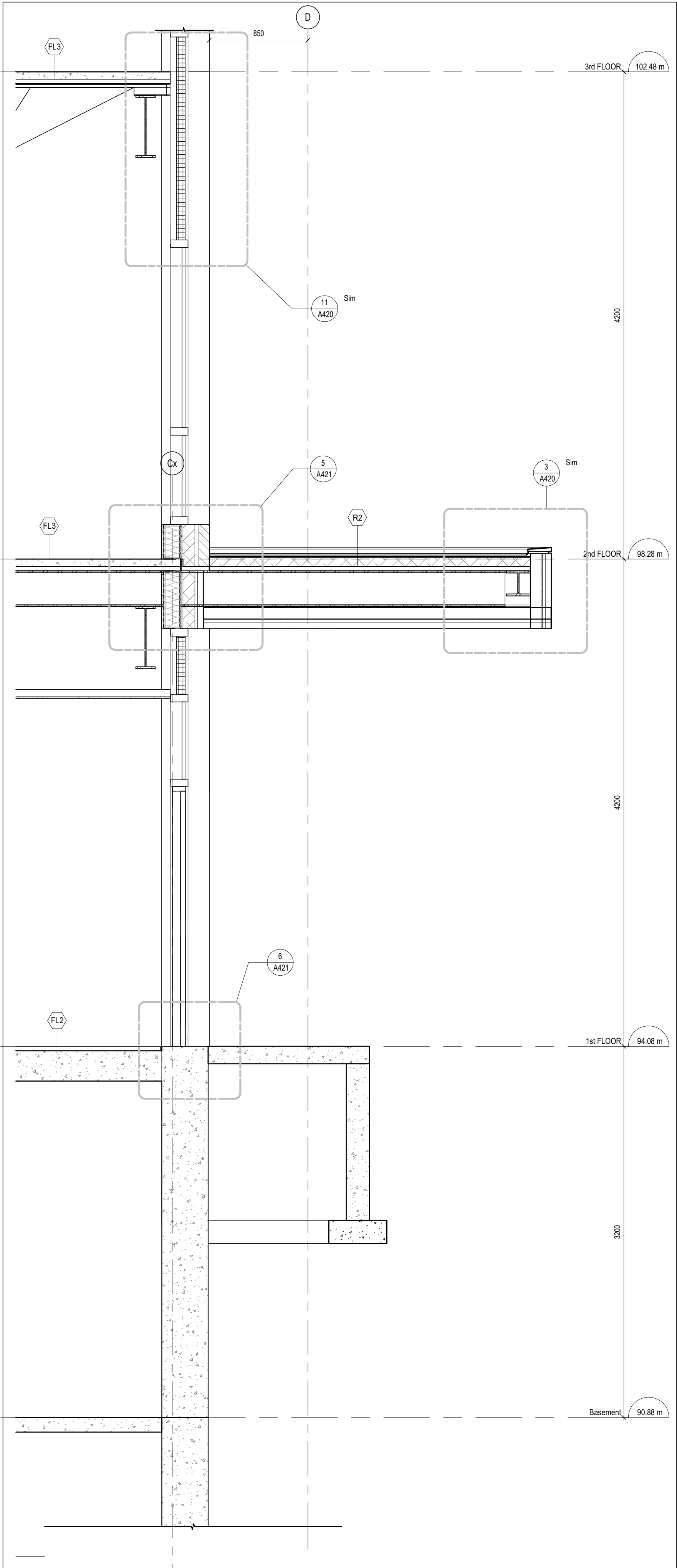
1 WALL SECTION A412 1:25
