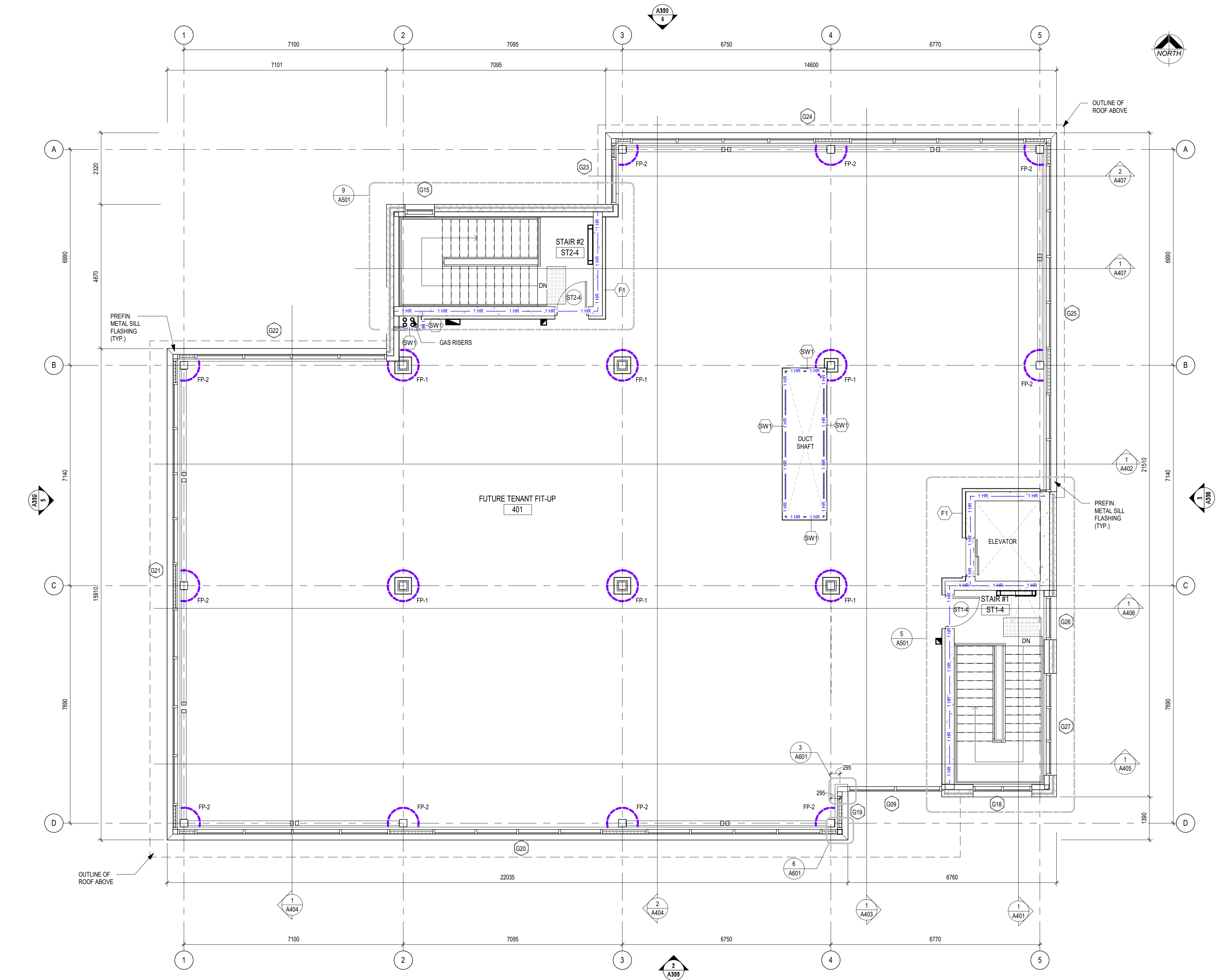
1 A205 4th FLOOR PLAN 1 : 75
