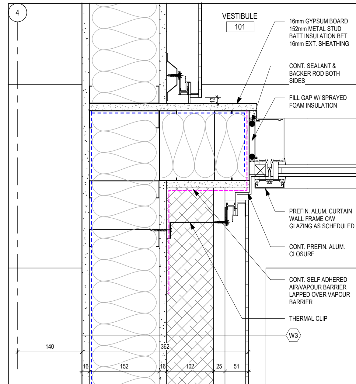
2 A601 PLAN DETAIL 1:5
