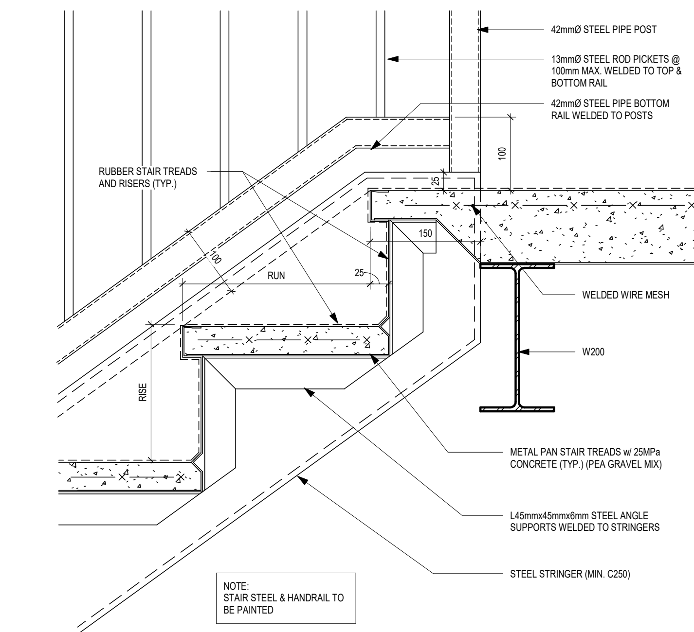
5 A504 TYP. STAIR DETAIL STEEL W/ CONC (TOP) 1 : 5
