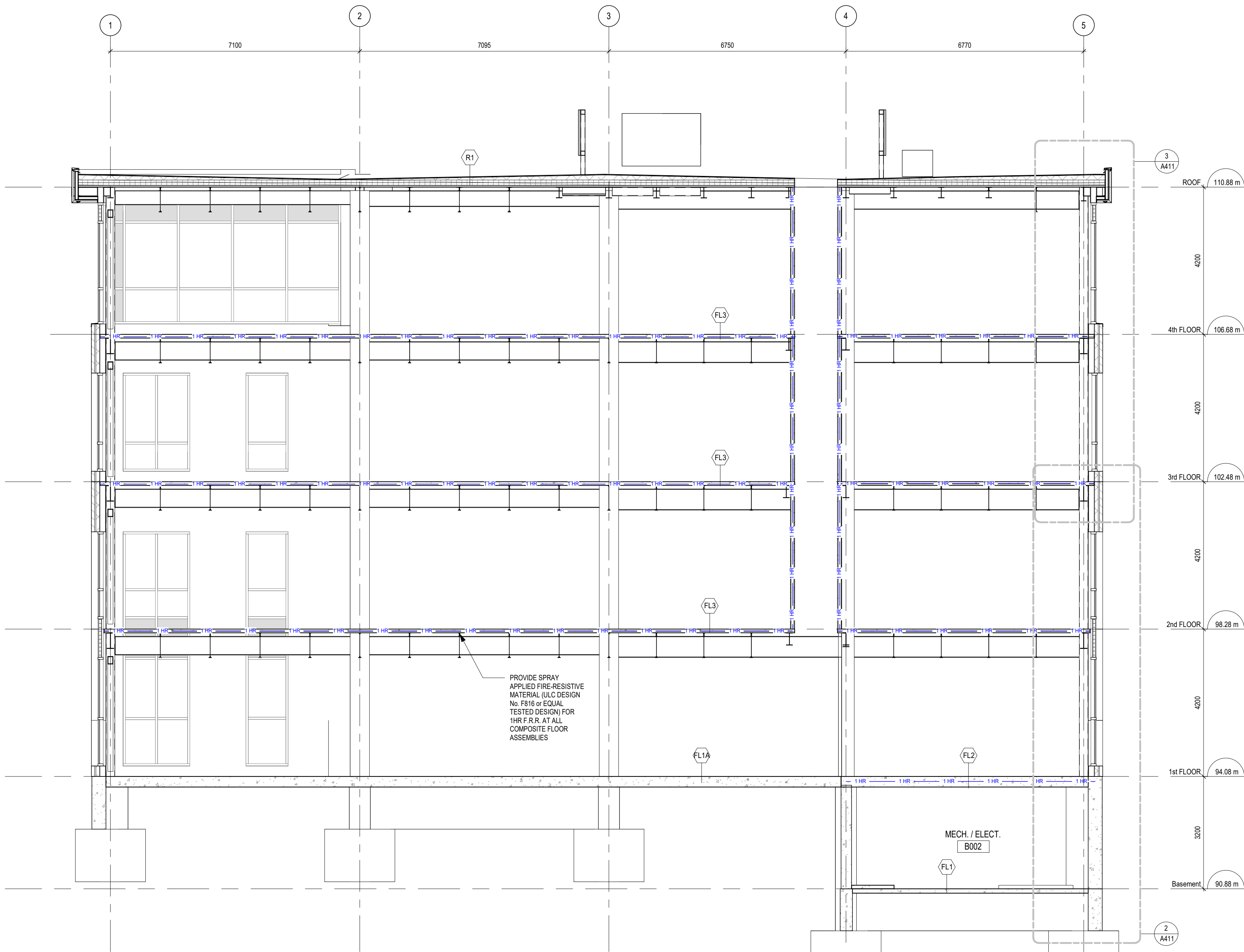
1 A402 BUILDING SECTION 1 : 75
