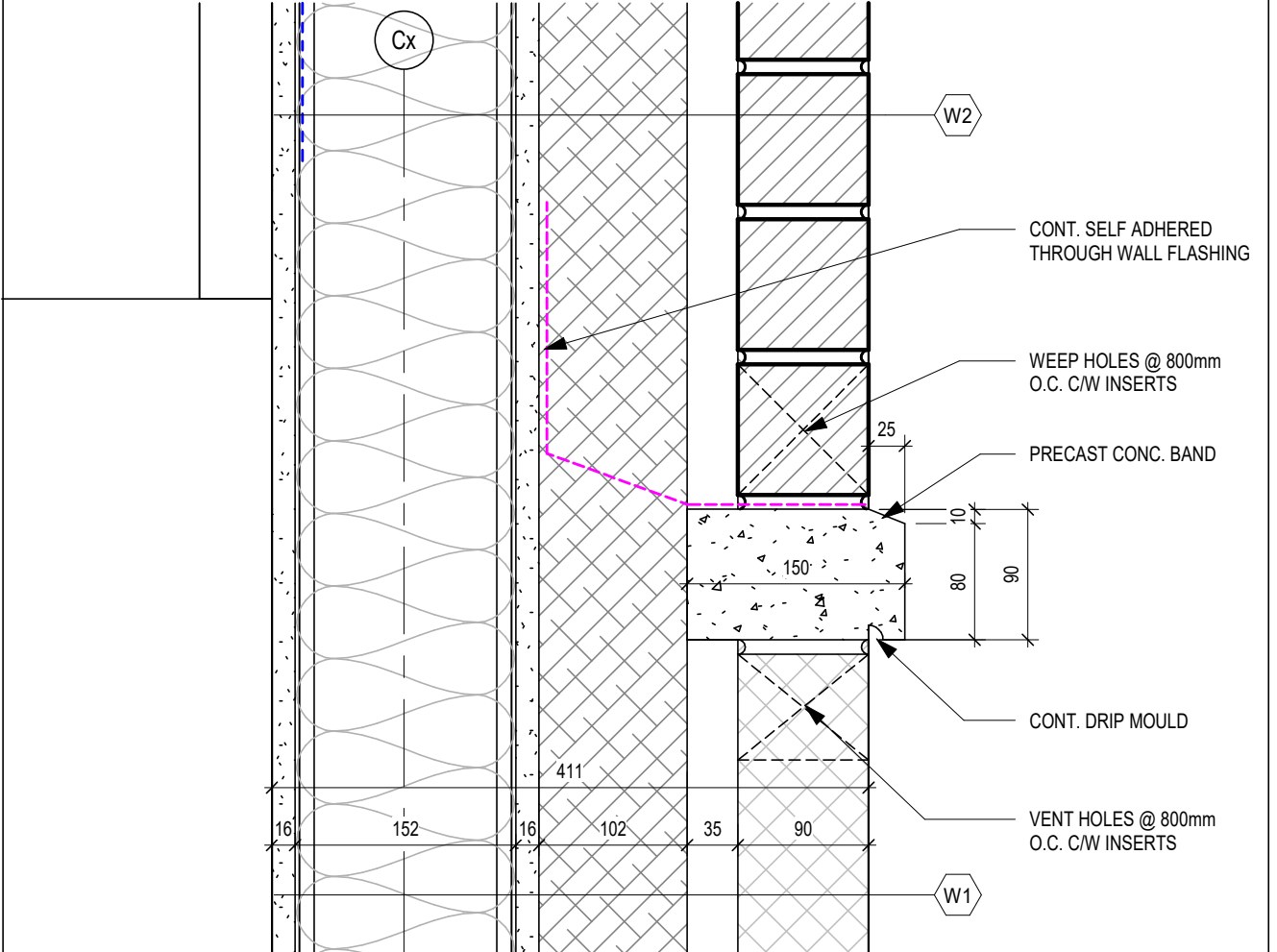
2 SECTION DETAIL A420 1:5
